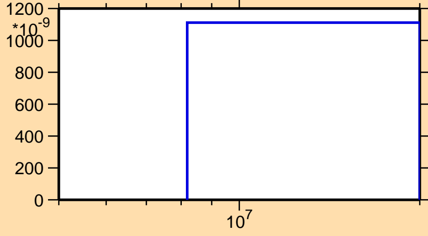
\sigma vs. E for ^{100}\text{Zr}(n,t)
