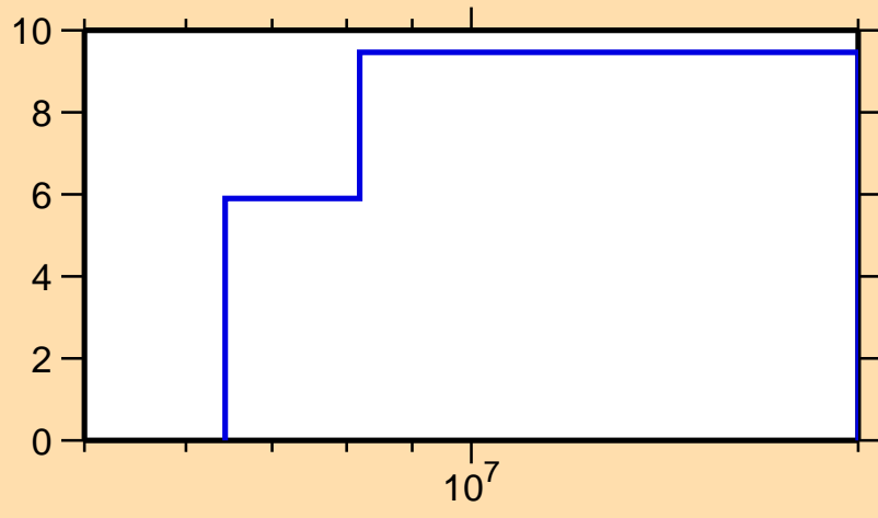
\Delta\sigma/\sigma vs. E for ^{100}\text{Zr}(n,\text{tot.})
