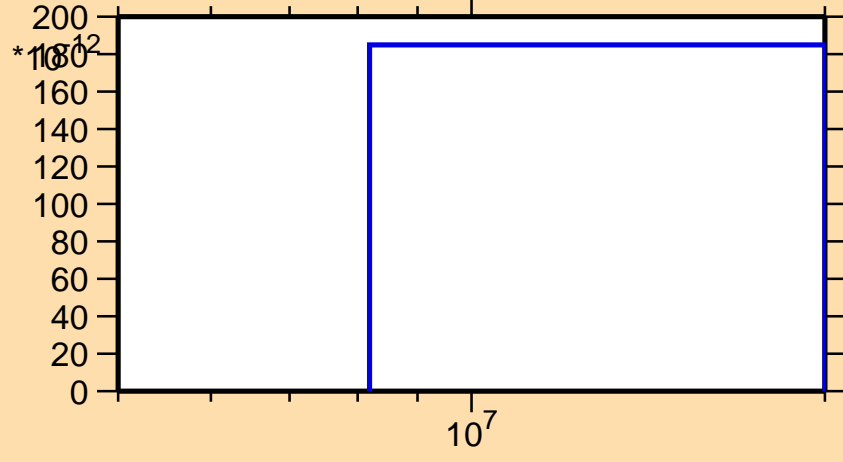
\sigma vs. E for ^{100}\text{Zr}(n,nt)
