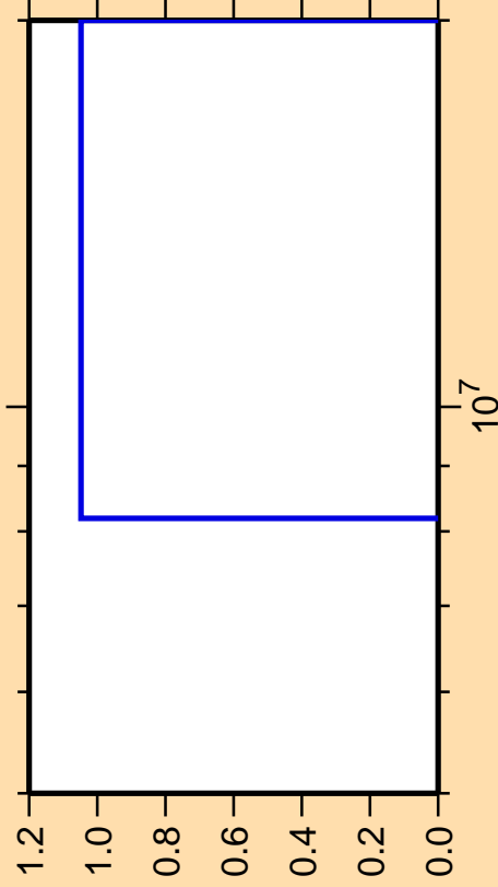
\Delta\sigma/\sigma vs. E for ^{100}\text{Zr}(n,nd)
