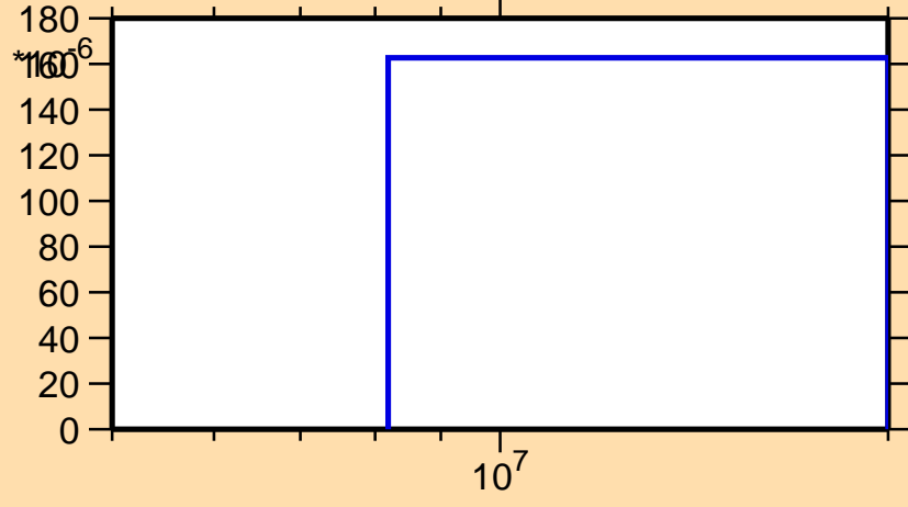
\sigma vs. E for ^{100}\text{Zr}(n,p)
