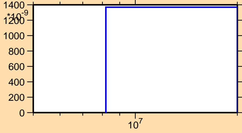
\sigma vs. E for ^{100}\text{Zr}(n,np)
