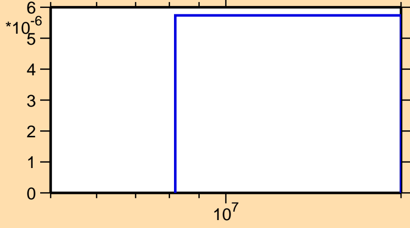
\sigma vs. E for ^{100}\text{Zr}(n,d)
