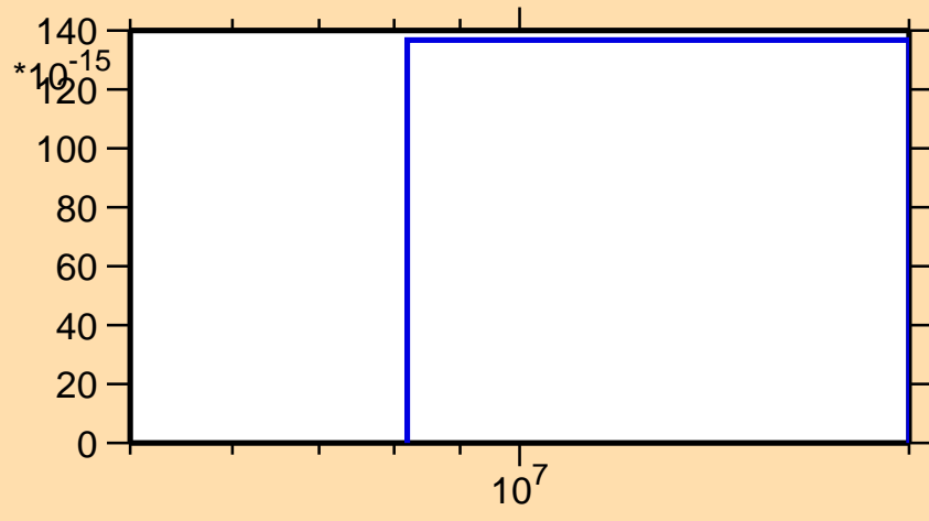
\sigma vs. E for ^{100}\text{Zr}(n,nd)
