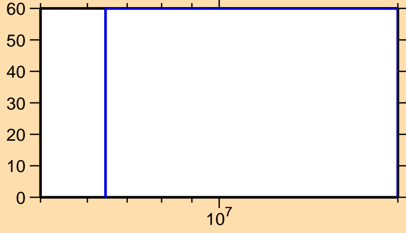
\Delta\sigma/\sigma vs. E for ^{100}\text{Zr}(n,\gamma)
