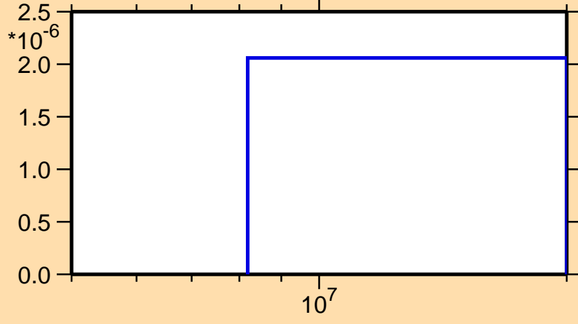
\sigma vs. E for ^{100}\text{Zr}(n,n\alpha)
