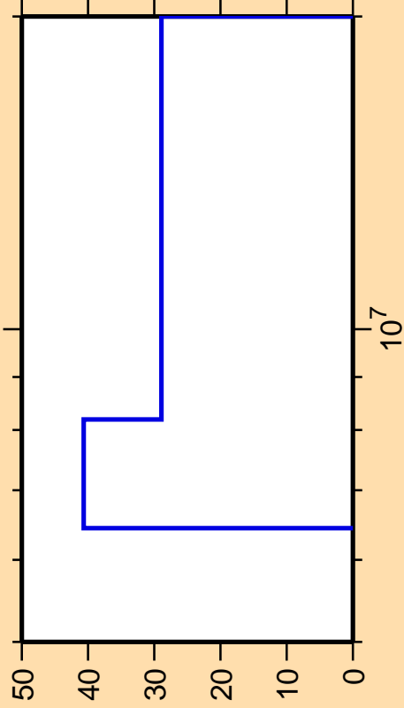
\Delta\sigma/\sigma vs. E for ^{100}\text{Zr}(n,2n)
