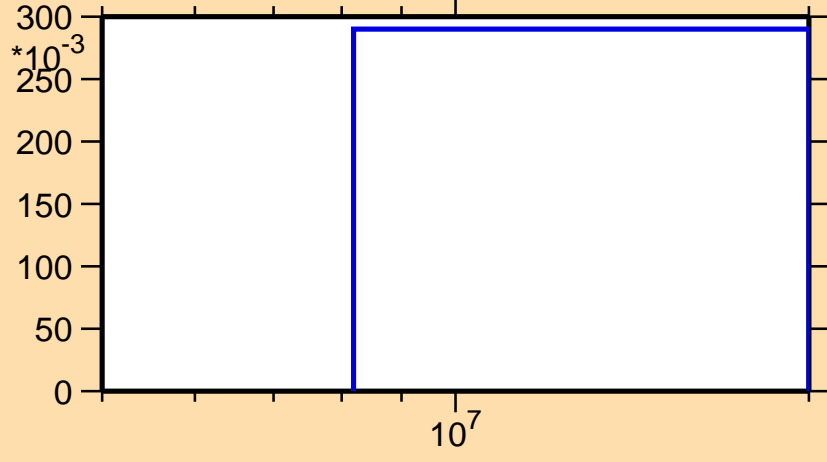
\sigma vs. E for ^{100}\text{Zr}(n,3n)
