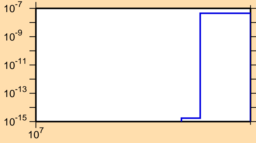
\sigma vs. E for ^{101}\text{Zr}(n,\text{nd})
