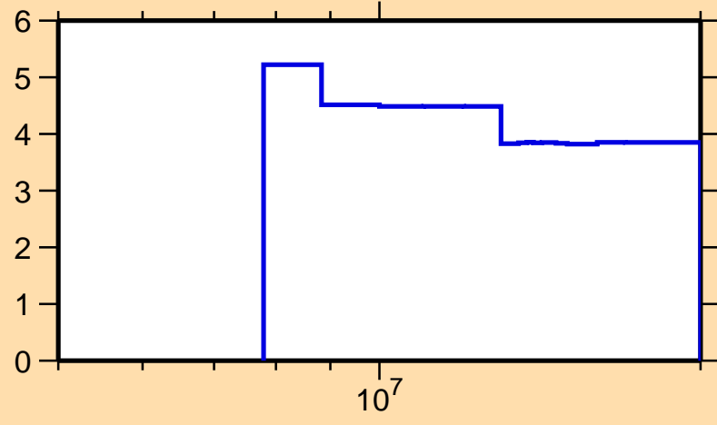
\Delta\sigma/\sigma vs. E for ^{101}\text{Zr}(n,\text{nonel.})
