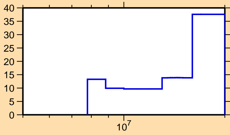
\Delta\sigma/\sigma vs. E for ^{101}\text{Zr}(n,2n)
