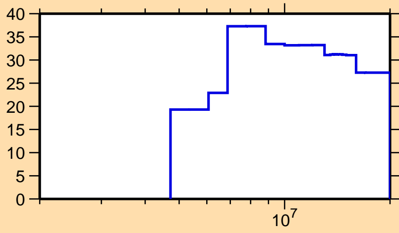
\Delta\sigma/\sigma vs. E for ^{101}\text{Zr}(n,\text{inel.})
