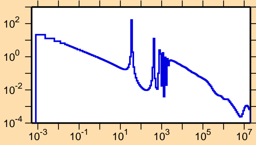
\sigma vs. E for ^{101}\text{Zr}(n,\gamma)
