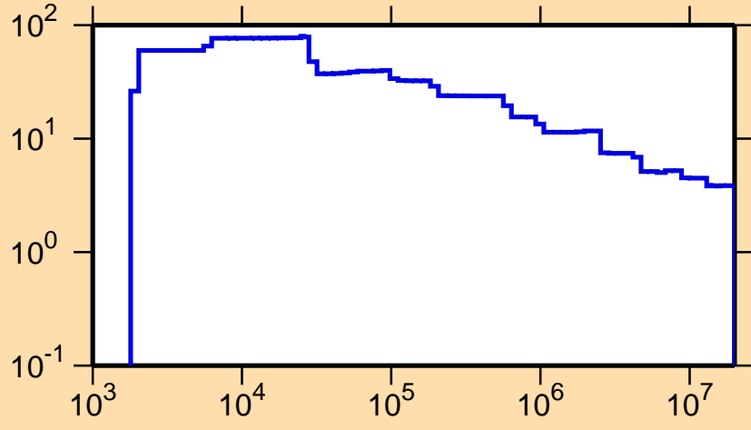
\Delta\sigma/\sigma vs. E for ^{101}\text{Zr}(n,\text{nonel.})
