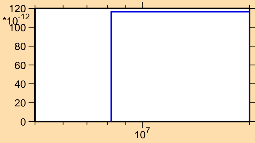
\sigma vs. E for ^{101}\text{Zr}(n,2n\alpha)
