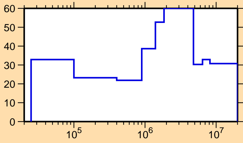
\Delta\sigma/\sigma vs. E for ^{101}\text{Zr}(n,n_1)
