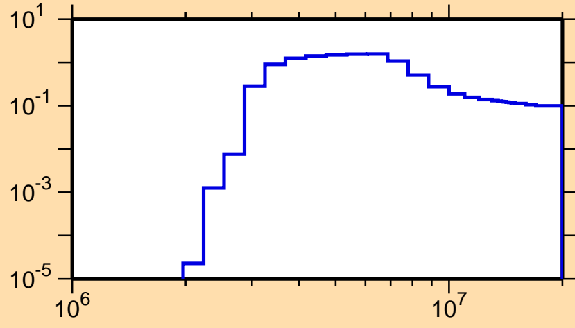
\sigma vs. E for ^{102}\text{Zr}(n,n\text{cont.})
