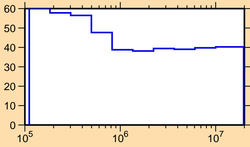
\Delta\sigma/\sigma vs. E for ^{102}\text{Zr}(n,n_1)
