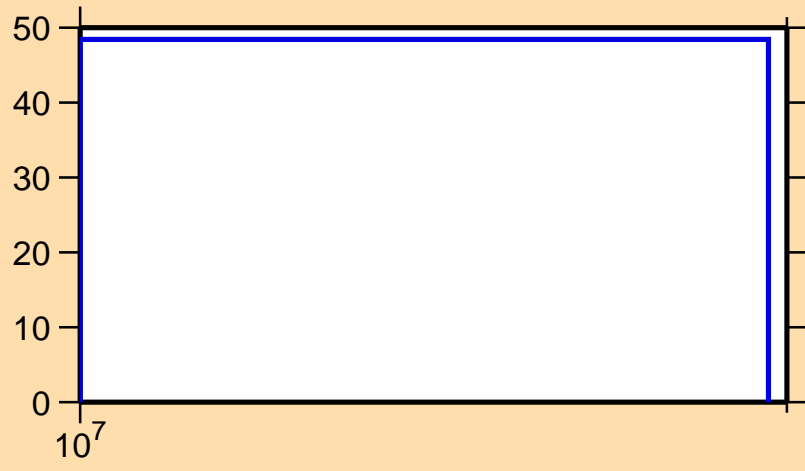
\Delta\sigma/\sigma vs. E for ^{102}\text{Zr}(n,el.)
