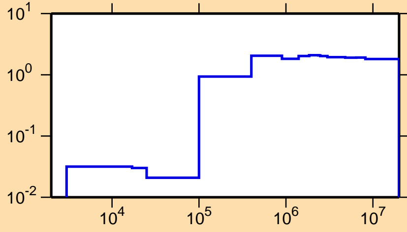
\sigma vs. E for ^{102}\text{Zr}(n,\text{nonel.})
