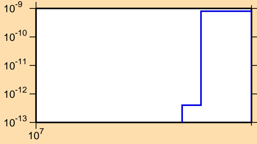
\sigma vs. E for ^{103}\text{Zr}(n,2n\alpha)
