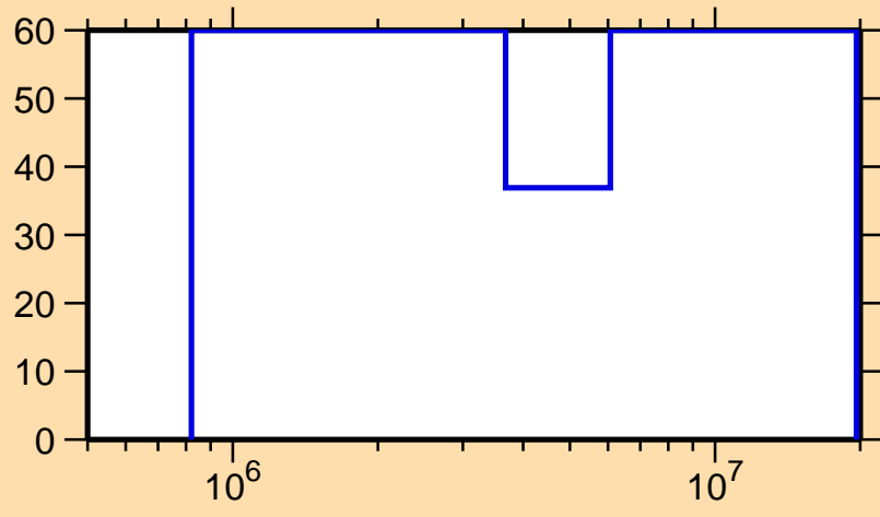
\Delta\sigma/\sigma vs. E for ^{103}\text{Zr}(n,n\text{cont.})
