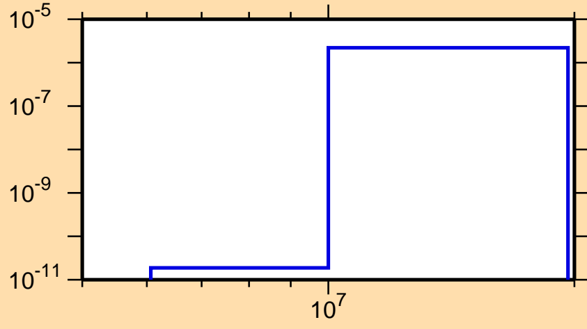
\sigma vs. E for ^{103}\text{Zr}(n,\alpha)
