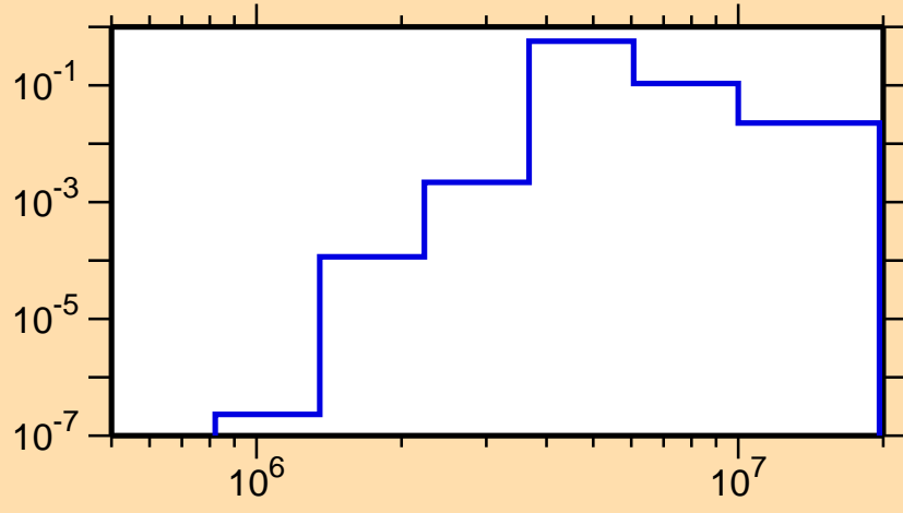
\sigma vs. E for ^{103}\text{Zr}(n,ncont.)
