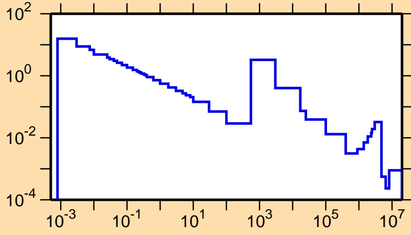
\sigma vs. E for ^{103}\text{Zr}(n,\gamma)
