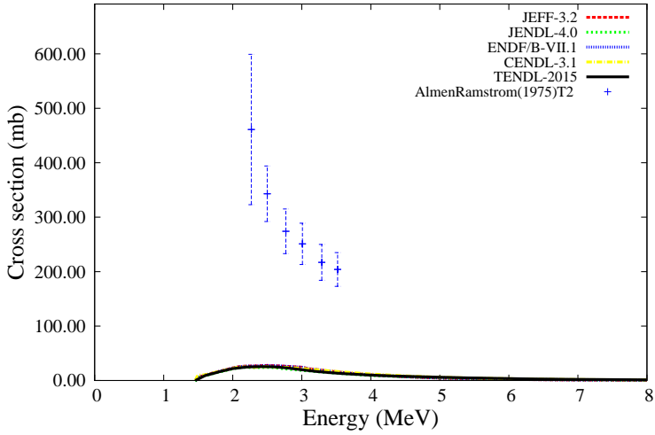
^{59}\text{Co}(n,g)^{60}\text{Co}
