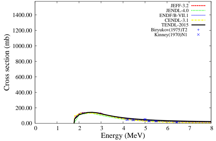
^{59}\text{Co}(n,g)^{60g}\text{Co}
