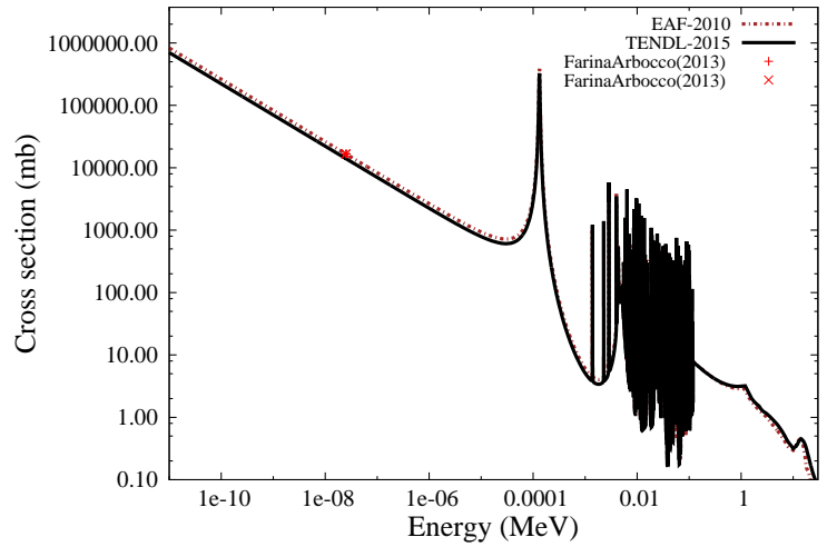
^{59}\text{Co}(n,g)^{60}\text{Co}
