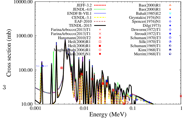
^{59}\text{Co}(n,g)^{60}\text{Co}
