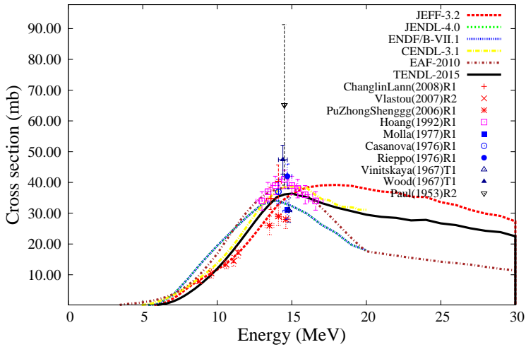
^{72}\text{Ge}(n,p)^{72}\text{Ga}
