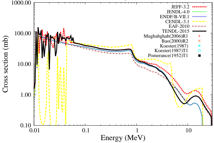
^{72}\text{Ge}(n,p)^{72}\text{Ga}
