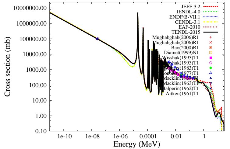
^{150}\text{Sm}(n,g)^{151}\text{Sm}
