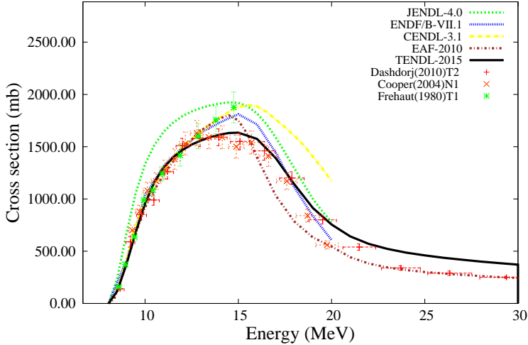
^{150}\text{Sm}(n,n_1')^{150}\text{Sm}
