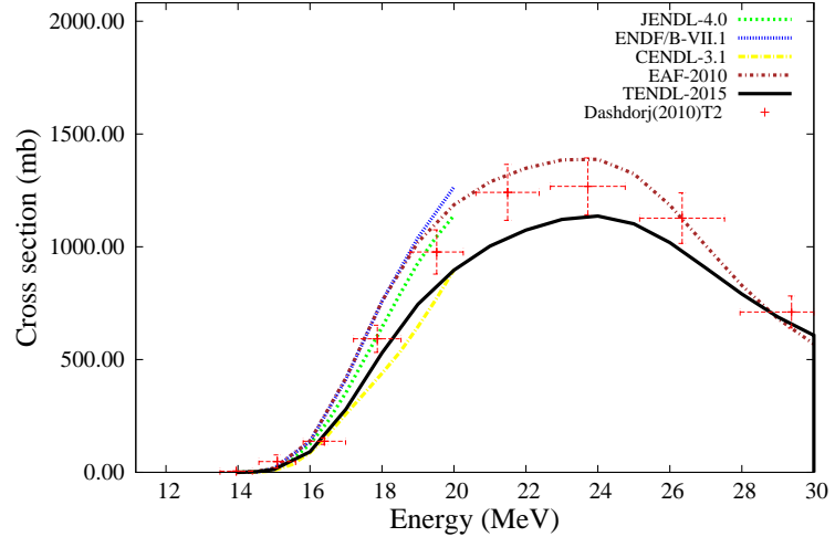
^{150}\text{Sm}(n,g)^{151}\text{Sm}
