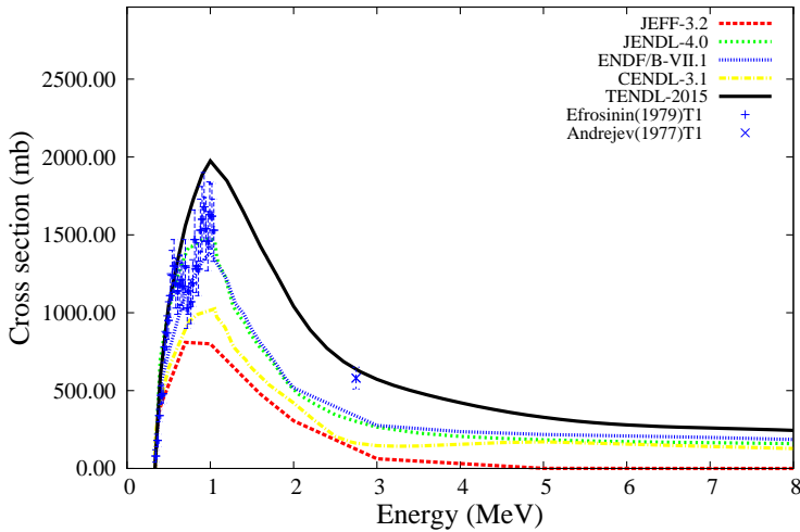
^{150}\text{Sm}(n,g)^{151}\text{Sm}
