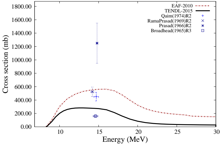
^{159}\text{Tb}(n,g)^{160}\text{Tb}
