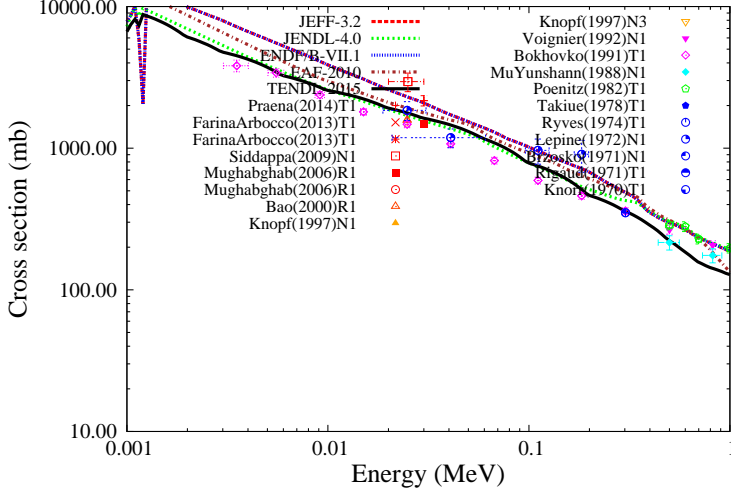
^{159}\text{Tb}(n,g)^{160}\text{Tb}
