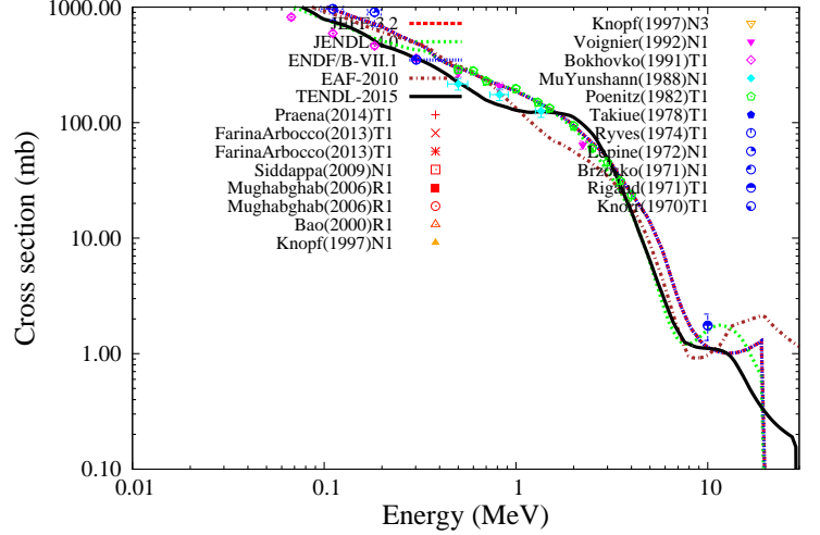
^{159}\text{Tb}(n,p)^{159}\text{Gd}
