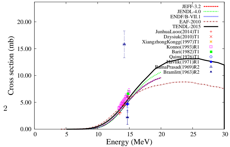
^{159}\text{Tb}(n,p)^{159}\text{Gd}
