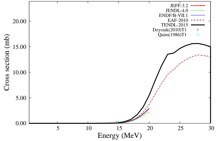
^{159}\text{Tb}(n,g)^{160}\text{Tb}
