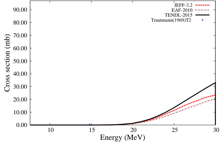
^{238}\text{U}(n,n_2')^{238}\text{U}
