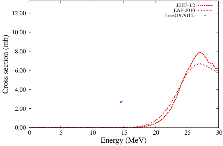
^{238}\text{U}(n,n_1')^{238}\text{U}
