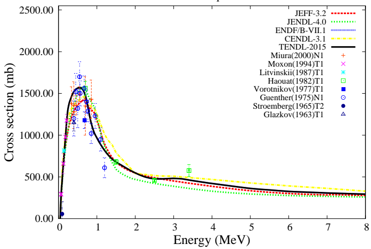
^{238}\text{U}(n,n_3')^{238}\text{U}
