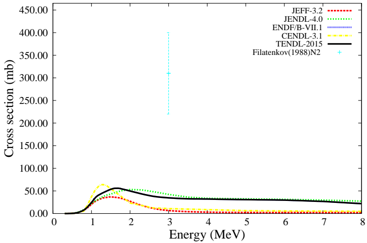
^{238}\text{U}(n,n_3')^{238}\text{U}
