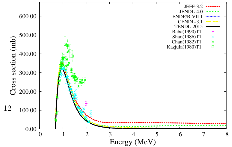
^{238}\text{U}(n,n_5')^{238}\text{U}
