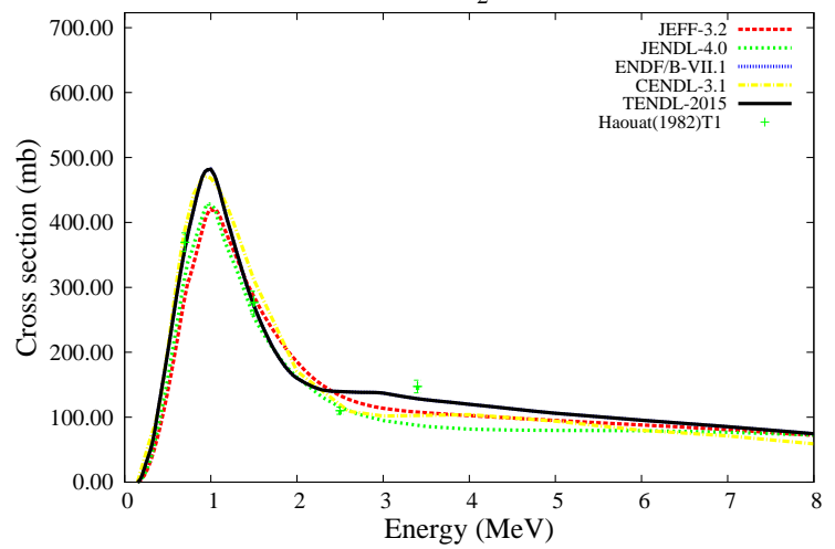
^{238}\text{U}(n,n_5')^{238}\text{U}
