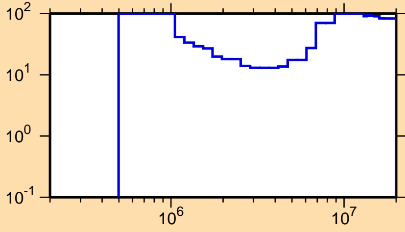
\Delta\sigma/\sigma vs. E for ^{222}\text{Ac}(n,n\text{cont.})
