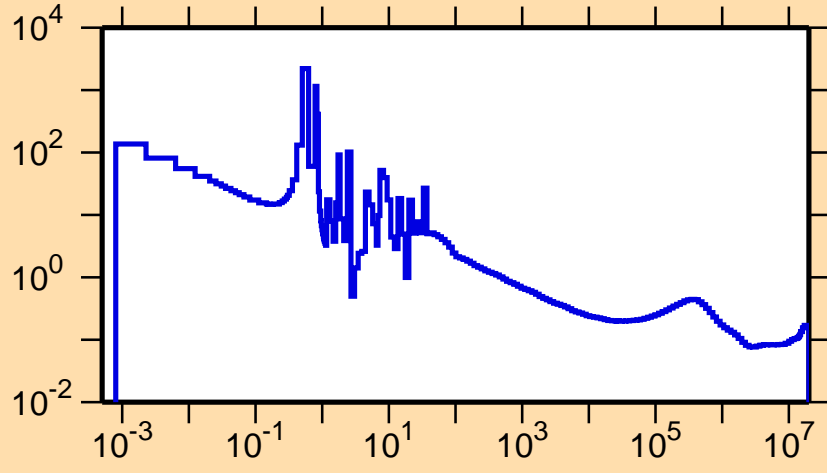
\sigma vs. E for ^{222}\text{Ac}(n,f)
