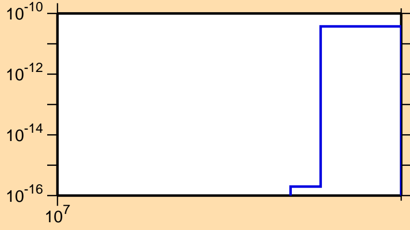
\sigma vs. E for ^{222}\text{Ac}(\text{mt } 11)
