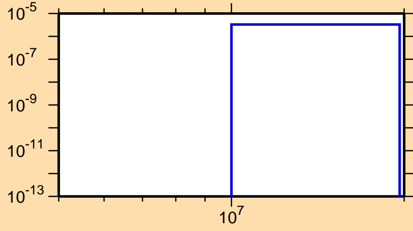
\sigma vs. E for ^{222}\text{Ac}(n,\text{nd})
