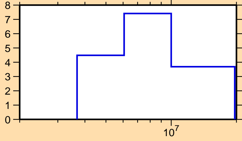
\Delta\sigma/\sigma vs. E for ^{222}\text{Ac}(n,\text{tot.})
