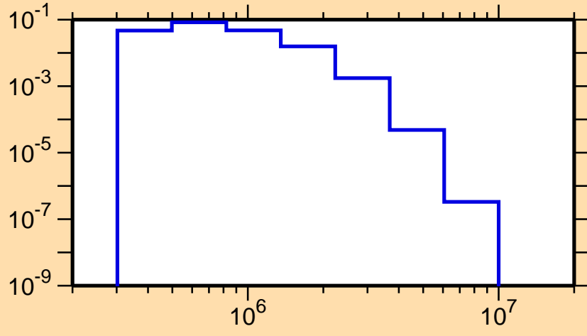
\sigma vs. E for ^{222}\text{Ac}(n,n_3)
