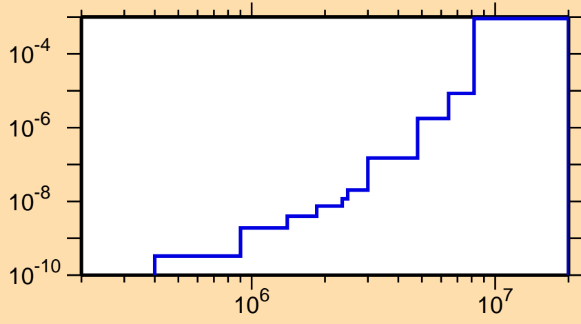
\sigma vs. E for ^{222}\text{Ac}(n,n\alpha)
