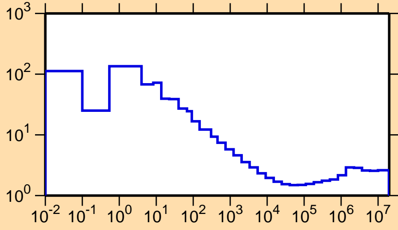
\sigma vs. E for ^{222}\text{Ac}(n,\text{nonel.})
