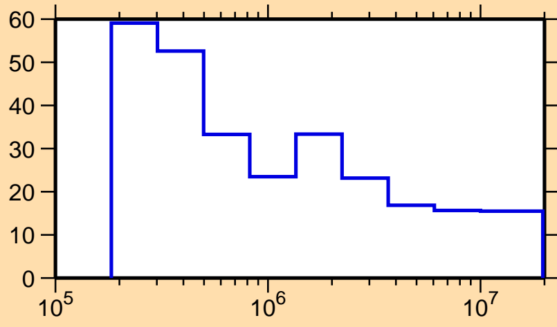
\Delta\sigma/\sigma vs. E for ^{222}\text{Ac}(n,\text{nonel.})
