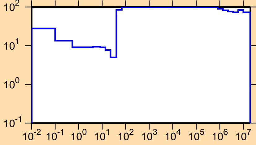
\Delta\sigma/\sigma vs. E for ^{222}\text{Ac}(n,\gamma)
