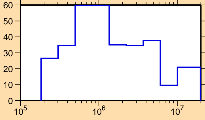
\Delta\sigma/\sigma vs. E for ^{222}\text{Ac}(n,\text{el.})
