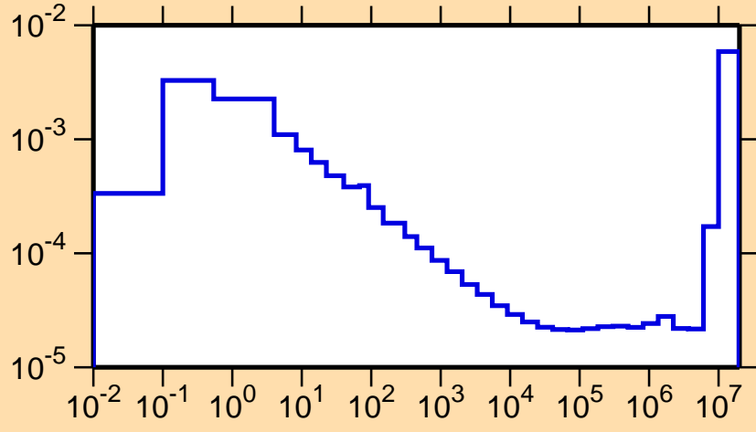
\sigma vs. E for ^{222}\text{Ac}(n,\alpha)
