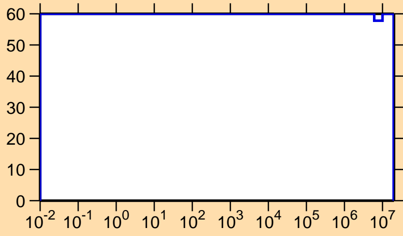
\Delta\sigma/\sigma vs. E for ^{222}\text{Ac}(n,p)
