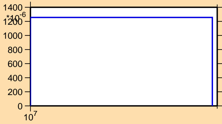
\sigma vs. E for ^{222}\text{Ac}(n,3n\alpha)
