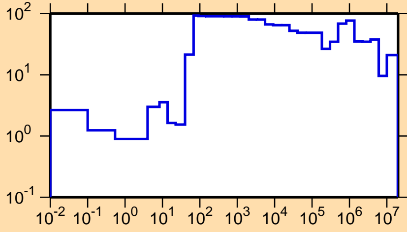
\Delta\sigma/\sigma vs. E for ^{222}\text{Ac}(n,el.)
