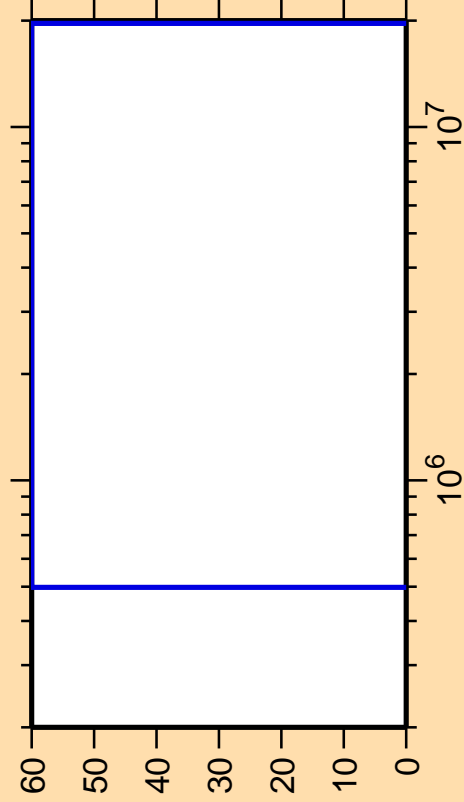
\Delta\sigma/\sigma vs. E for ^{222}\text{Ac}(n,n\alpha)
