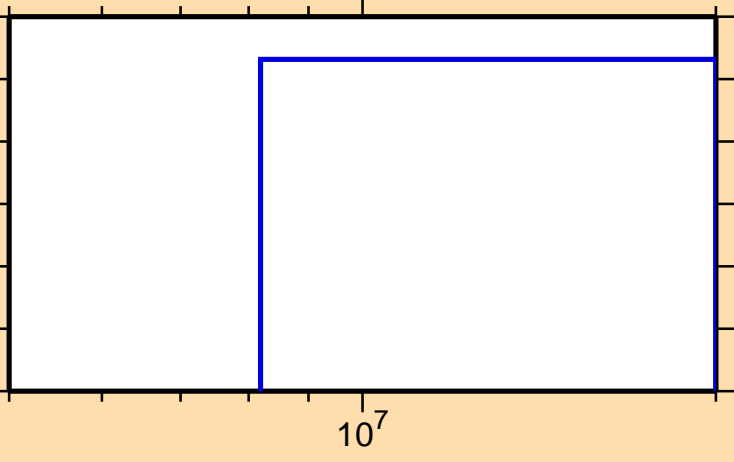
\sigma vs. E for ^{222}\text{Ac}(\text{mt } 42)
