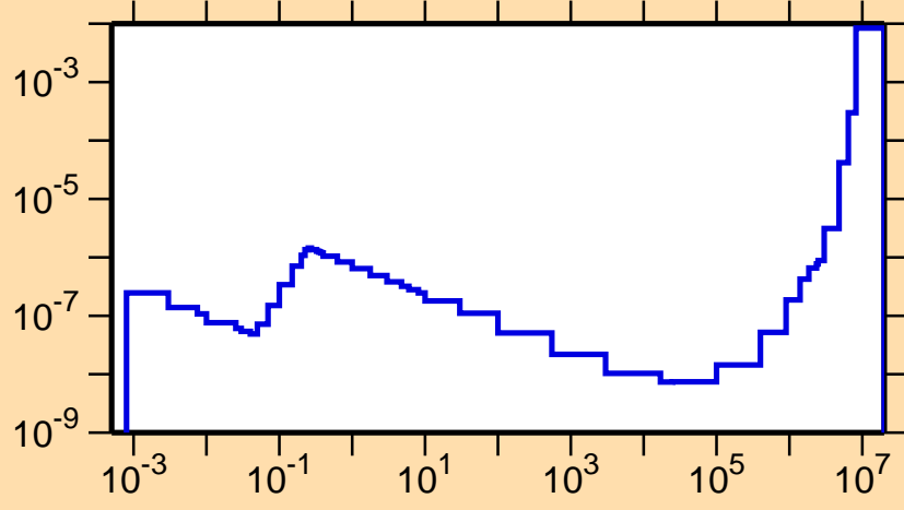
\sigma vs. E for ^{222}\text{Ac}(n,p)
