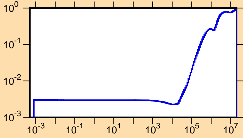
\mu vs. E for ^{223}\text{Ac}(\text{mt251})
