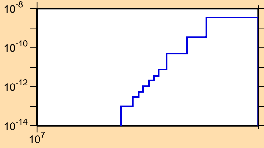
\sigma vs. E for ^{223}\text{Ac}(n,\text{He3})
