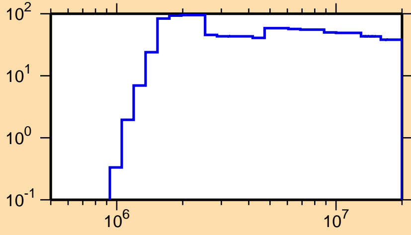
\Delta\sigma/\sigma vs. E for ^{223}\text{Ac}(n,p)
