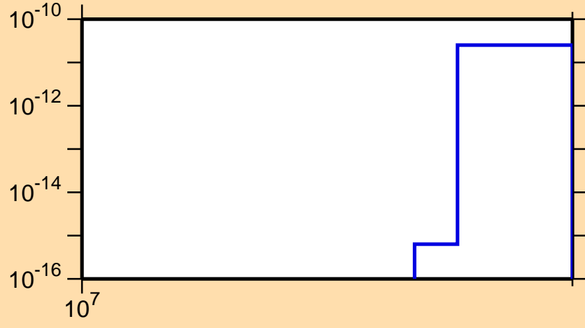
\sigma vs. E for ^{223}\text{Ac}(\text{mt } 11)
