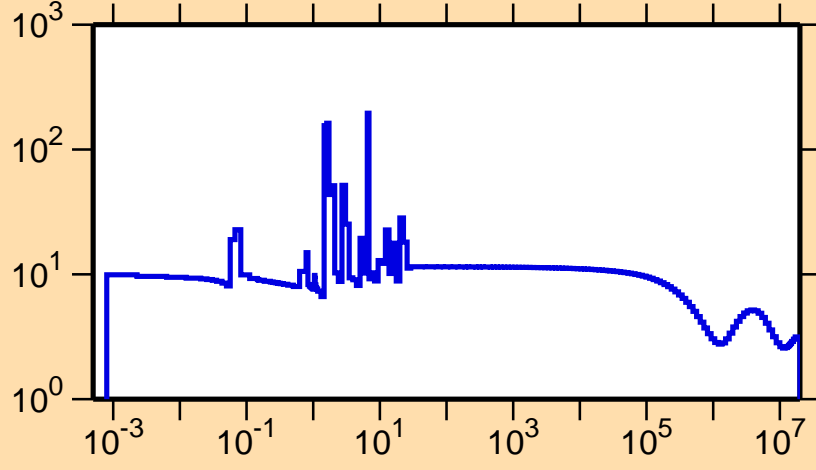
\sigma vs. E for ^{223}\text{Ac}(n,\text{el.})
