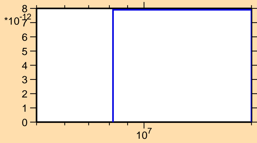
\sigma vs. E for ^{223}\text{Ac}(\text{mt } 45)
