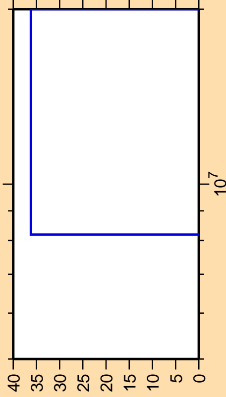
\Delta\sigma/\sigma vs. E for ^{223}\text{Ac}(\text{mt } 45)
