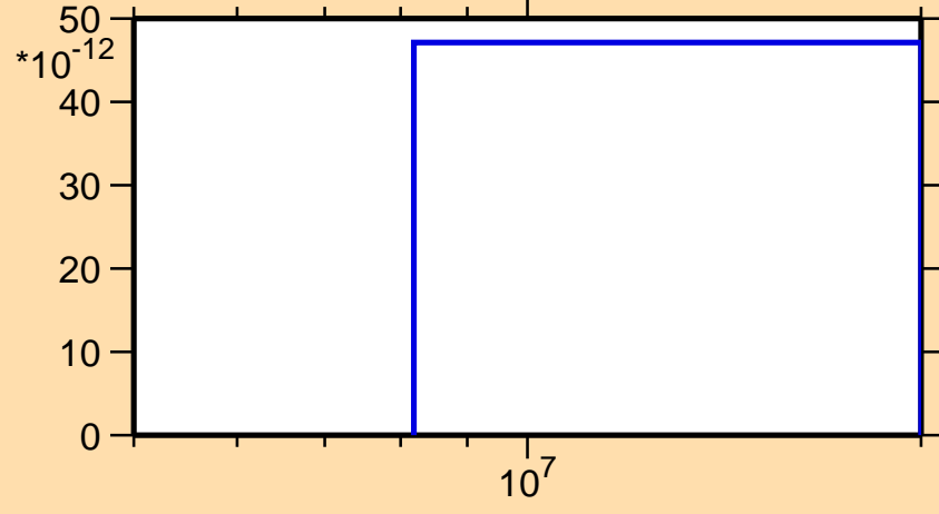
\sigma vs. E for ^{223}\text{Ac}(n,p\alpha)
