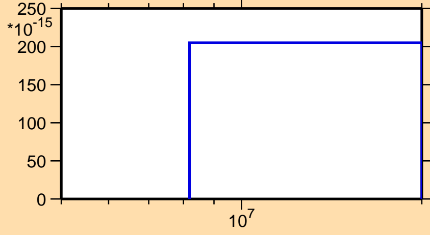
\sigma vs. E for ^{223}\text{Ac}(\text{mt } 11)
