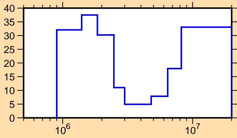
\Delta\sigma/\sigma vs. E for ^{223}\text{Ac}(n,\text{inel.})
