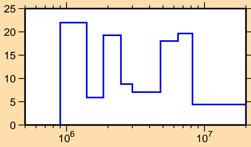
\Delta\sigma/\sigma vs. E for ^{223}\text{Ac}(n,\text{tot.})
