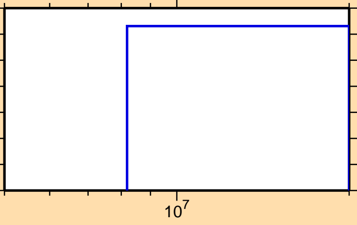
\sigma vs. E for ^{223}\text{Ac}(\text{mt } 34)
