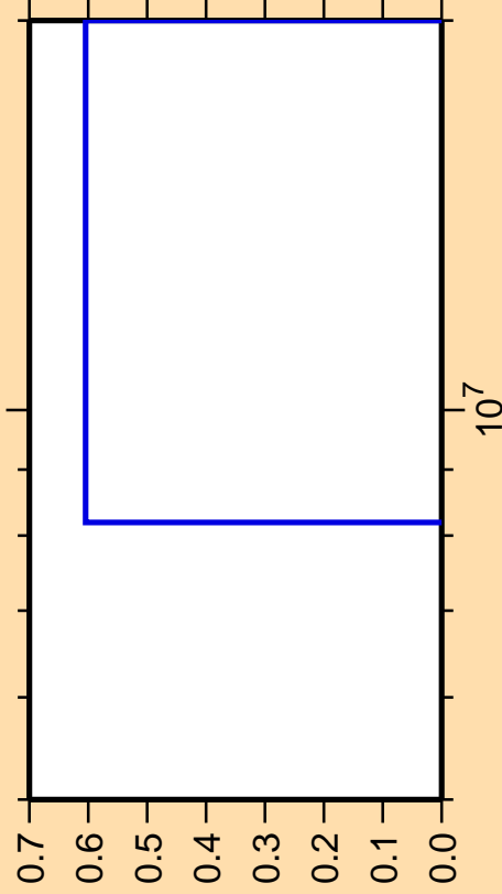
\Delta\sigma/\sigma vs. E for ^{223}\text{Ac}(\text{mt } 11)
