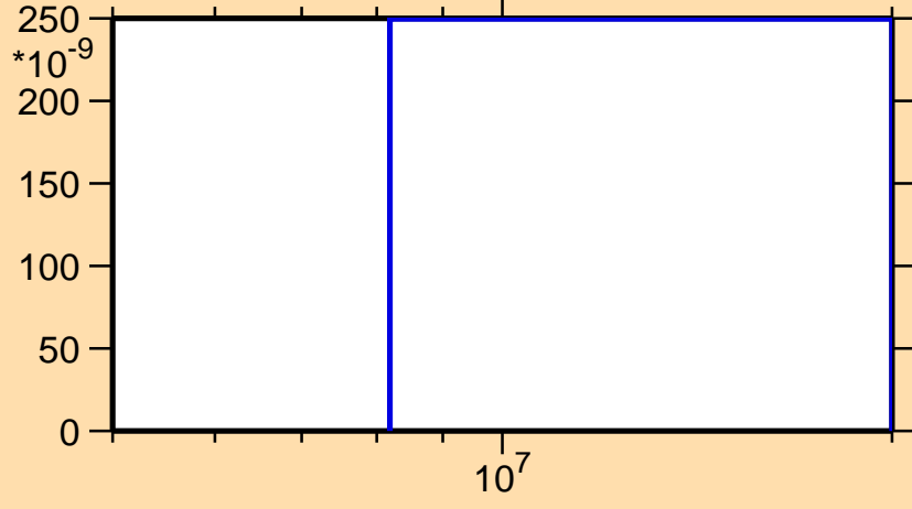
\sigma vs. E for ^{223}\text{Ac}(n,2np)
