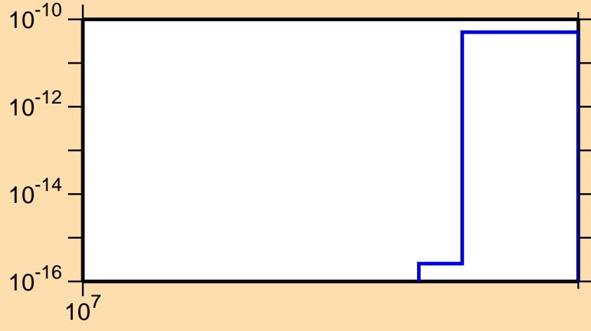
\sigma vs. E for ^{224}\text{Ac}(\text{mt 11})
