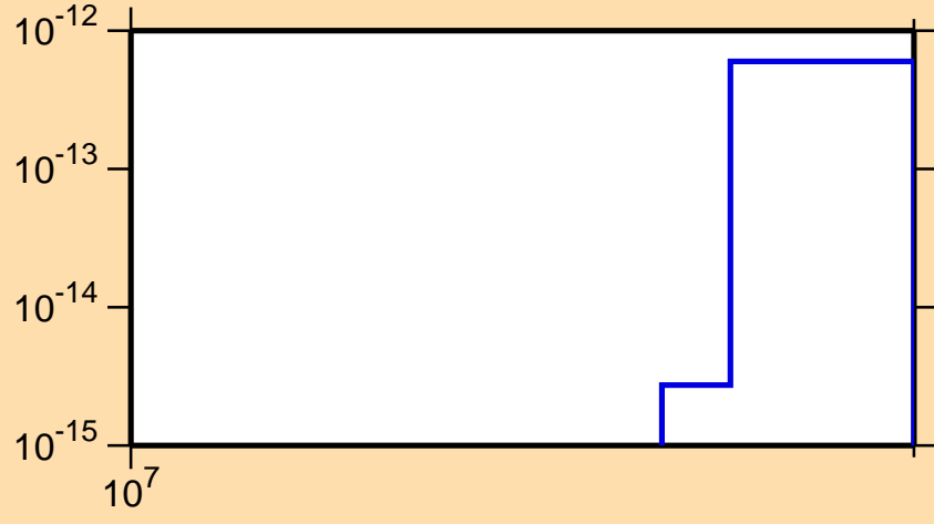
\sigma vs. E for ^{224}\text{Ac}(\text{mt } 34)
