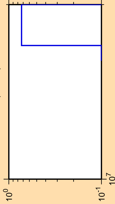
\Delta\sigma/\sigma vs. E for ^{224}\text{Ac}(\text{mt } 34)
