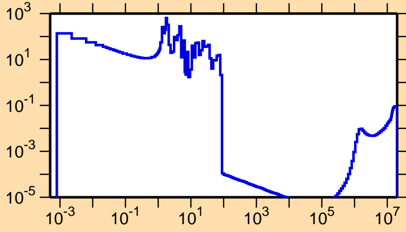
\sigma vs. E for ^{224}\text{Ac}(n,f)
