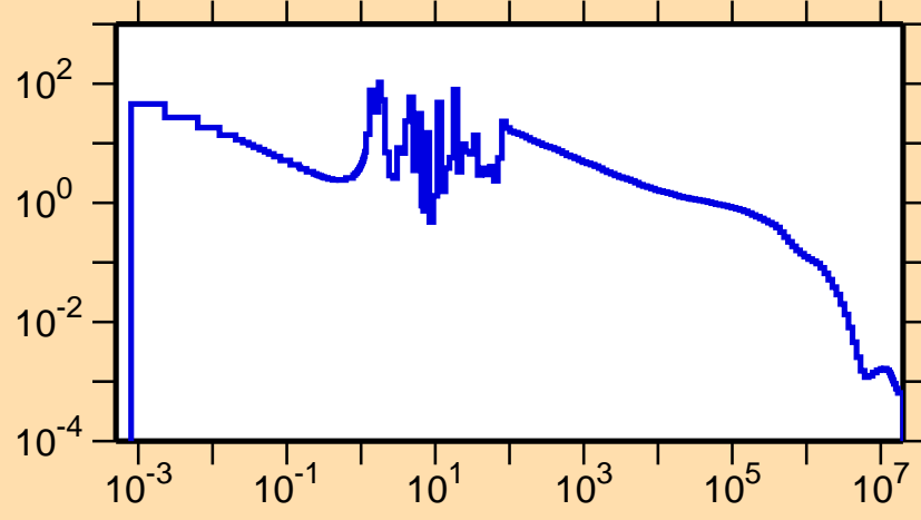
\sigma vs. E for ^{224}\text{Ac}(n,\gamma)
