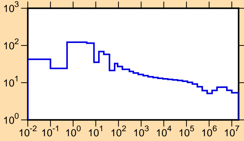
\sigma vs. E for ^{224}\text{Ac}(n,\text{tot.})
