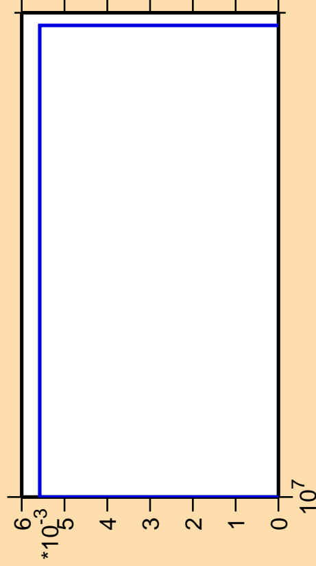
\Delta\sigma/\sigma vs. E for ^{224}\text{Ac} (mt 34)
