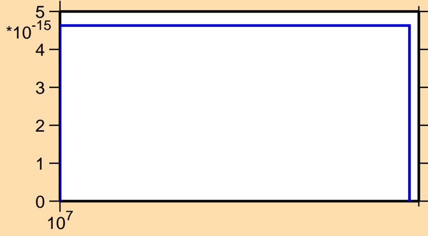
\sigma vs. E for ^{224}\text{Ac} (mt 34)
