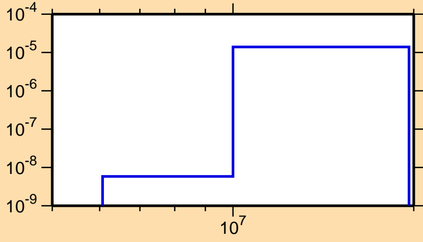
\sigma vs. E for ^{224}\text{Ac}(n,2n\alpha)
