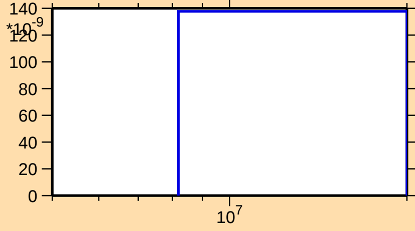
\sigma vs. E for ^{225}\text{Ac}(n,\text{nd})
