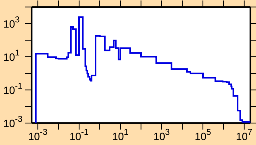
\sigma vs. E for ^{225}\text{Ac}(n,\gamma)
