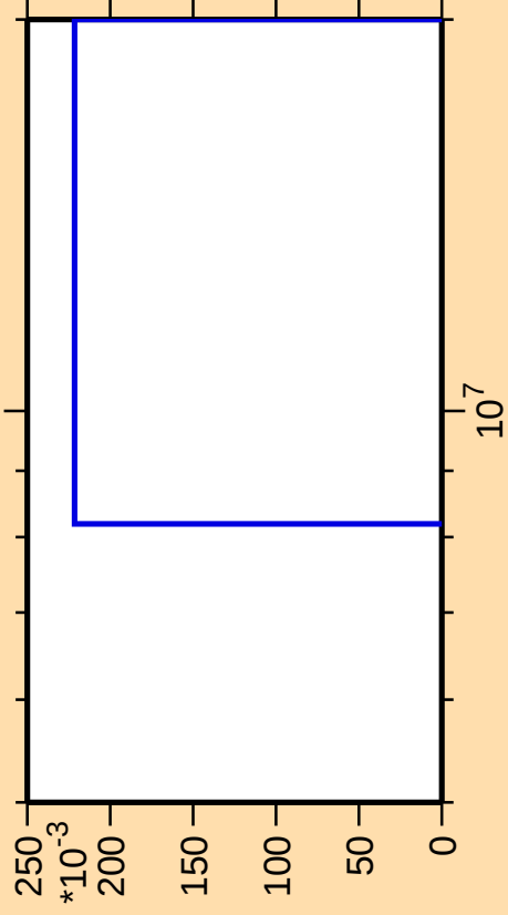
\Delta\sigma/\sigma vs. E for ^{225}\text{Ac}(\text{mt } 45)
