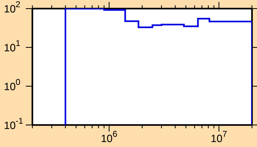
\Delta\sigma/\sigma vs. E for ^{225}\text{Ac}(n,n\text{cont.})
