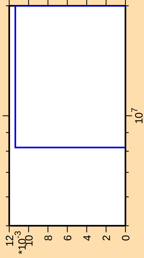
\Delta\sigma/\sigma vs. E for ^{225}\text{Ac}(\text{mt } 42)
