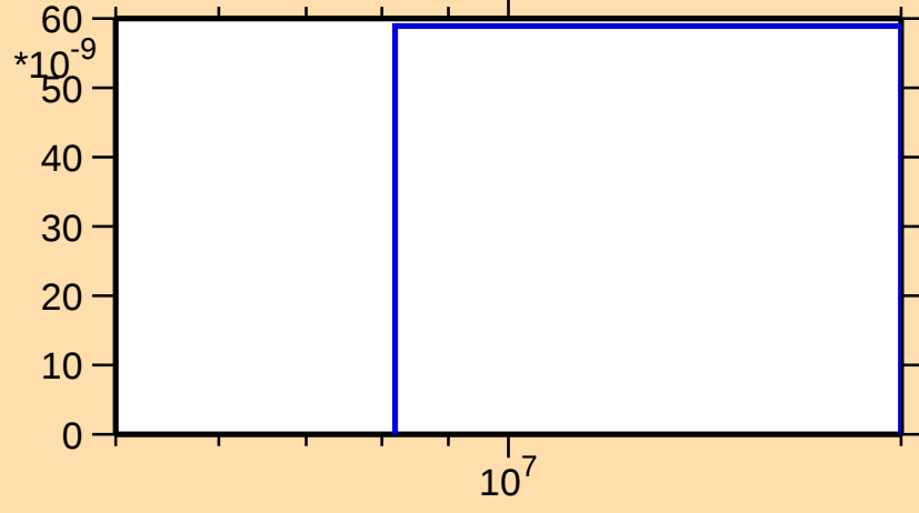
\sigma vs. E for ^{225}\text{Ac}(n,2np)
