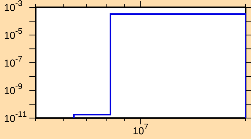
\sigma vs. E for ^{225}\text{Ac}(n,np)
