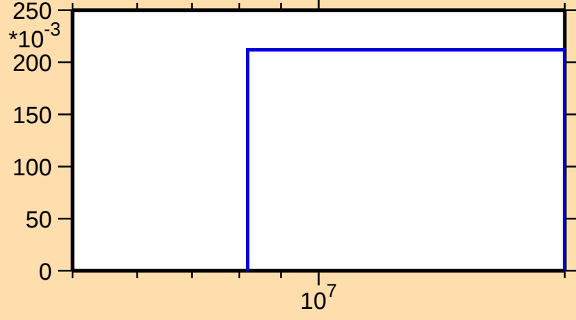
\sigma vs. E for ^{225}\text{Ac}(n,3n)
