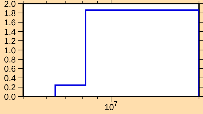
\sigma vs. E for ^{225}\text{Ac}(n,2n)
