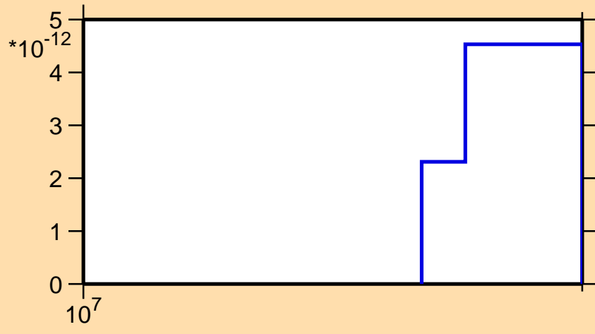
\sigma vs. E for ^{226}\text{Ac}(n,p\alpha)
