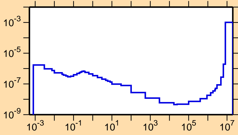
\sigma vs. E for ^{226}\text{Ac}(n,\alpha)
