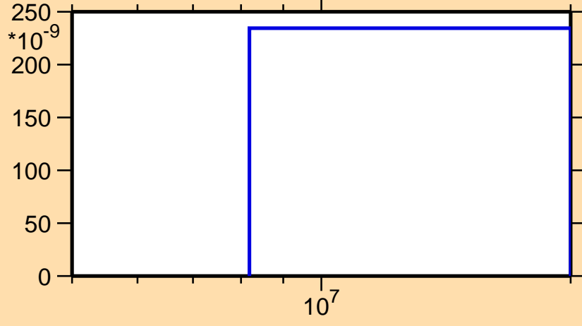
\sigma vs. E for ^{226}\text{Ac}(n,2np)
