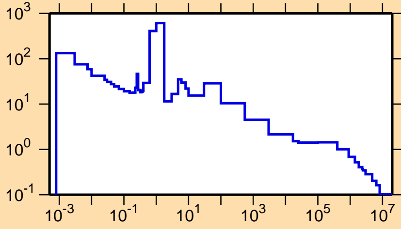
\sigma vs. E for ^{226}\text{Ac}(n,f)
