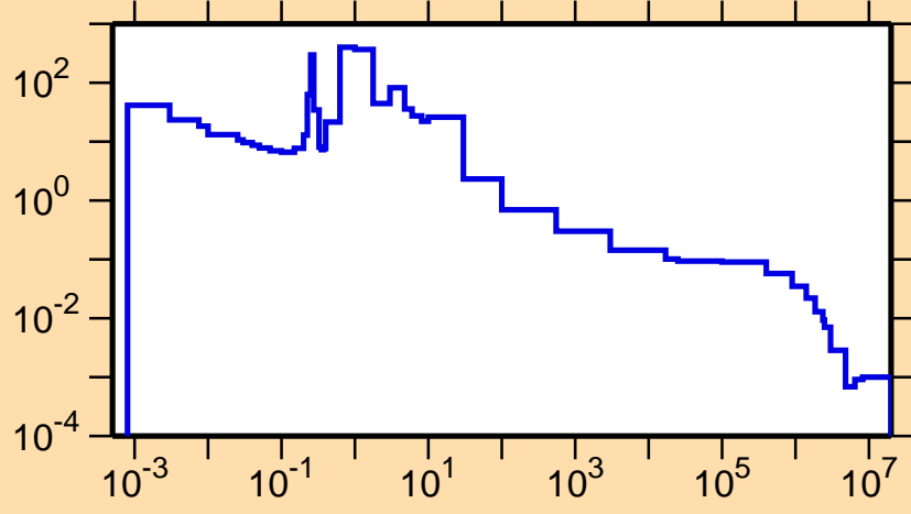
\sigma vs. E for ^{226}\text{Ac}(n,\gamma)
