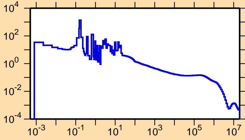
\sigma vs. E for ^{228}\text{Ac}(n,\gamma)
