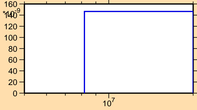
\sigma vs. E for ^{228}\text{Ac}(n,2n\alpha)
