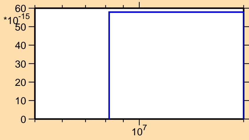
\sigma vs. E for ^{228}\text{Ac}(\text{mt } 11)
