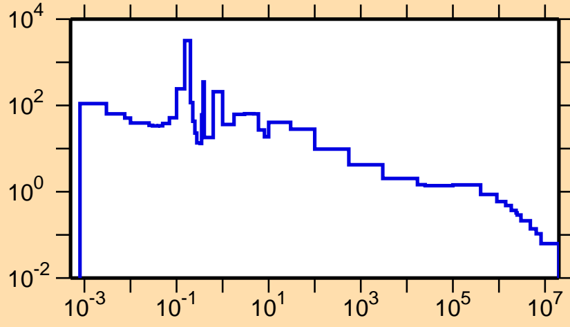
\sigma vs. E for ^{228}\text{Ac}(n,f)
