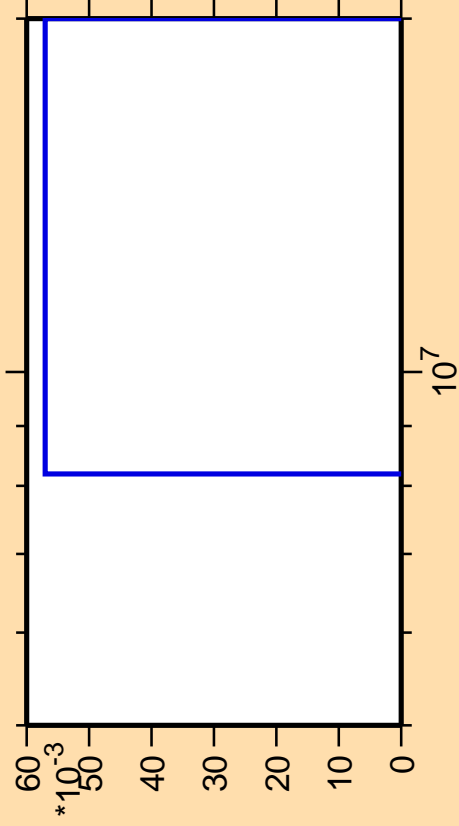
\Delta\sigma/\sigma vs. E for ^{228}\text{Ac}(\text{mt } 11)
