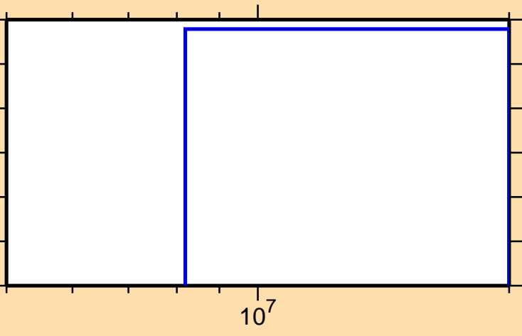
\sigma vs. E for ^{228}\text{Ac}(\text{mt } 11)
