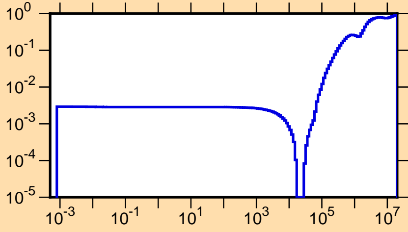
\mu vs. E for ^{229}\text{Ac}(\text{mt251})
