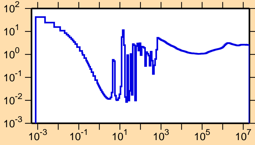
\sigma vs. E for ^{229}\text{Ac}(n,\text{nonel.})
