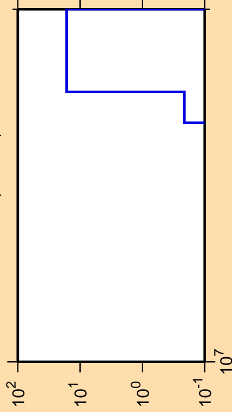
\Delta\sigma/\sigma vs. E for ^{229}\text{Ac}(n,\text{He3})
