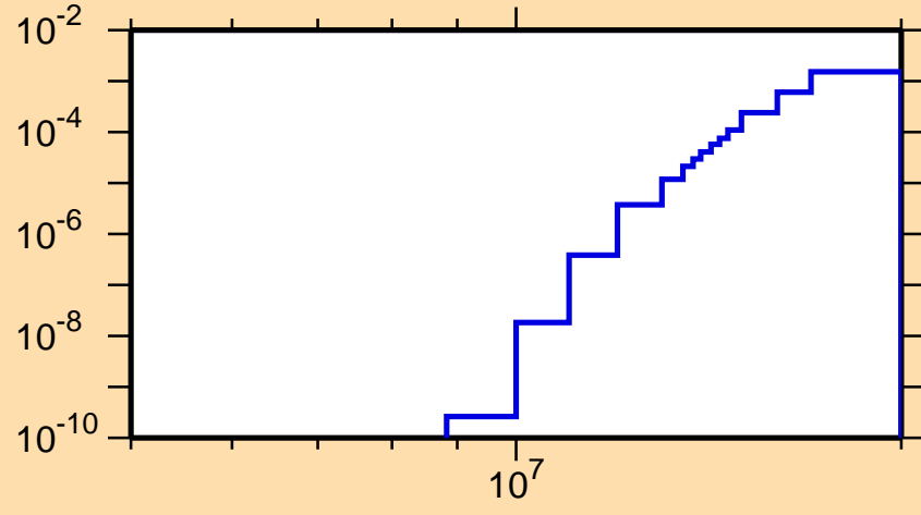
\sigma vs. E for ^{229}\text{Ac}(n,np)
