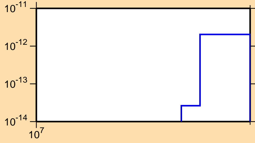
\sigma vs. E for ^{229}\text{Ac}(n,\text{He3})
