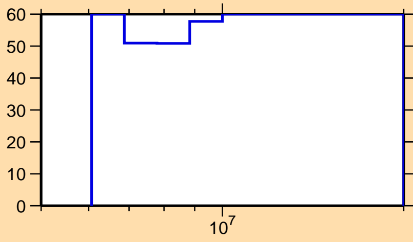
\Delta\sigma/\sigma vs. E for ^{229}\text{Ac}(n,2n)
