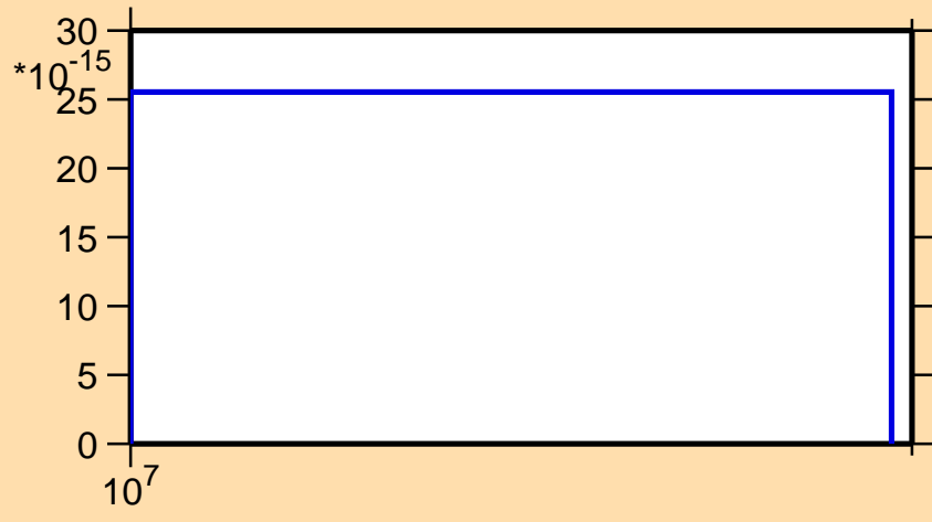
\sigma vs. E for ^{229}\text{Ac}(\text{mt } 11)
