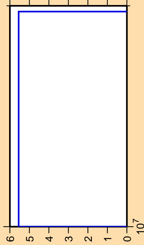
\Delta\sigma/\sigma vs. E for ^{229}\text{Ac}(n,3n\alpha)
