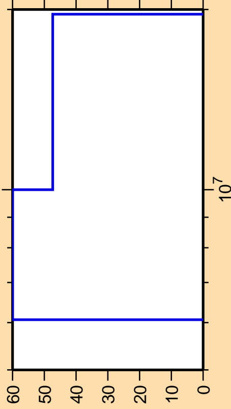
\Delta\sigma/\sigma vs. E for ^{229}\text{Ac}(n,d)
