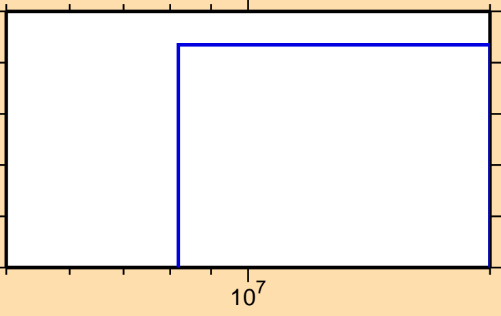
\sigma vs. E for ^{229}\text{Ac}(n,np)
