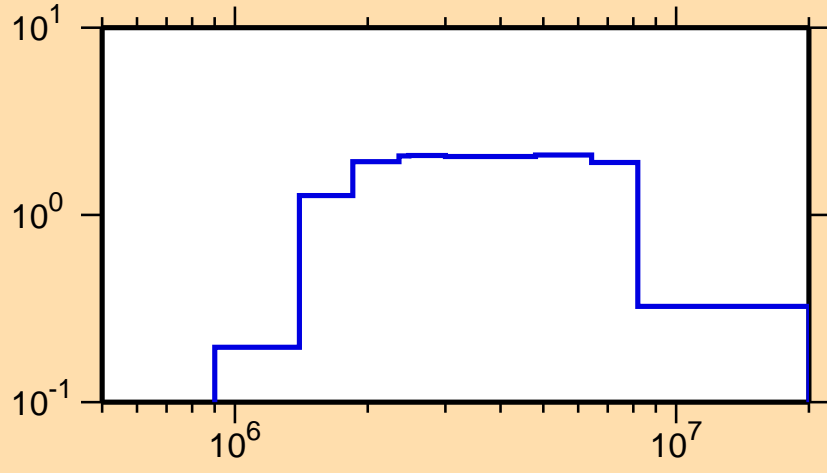
\sigma vs. E for ^{229}\text{Ac}(n,n\text{cont.})
