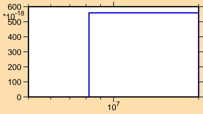
\sigma vs. E for ^{229}\text{Ac}(\text{mt } 42)
