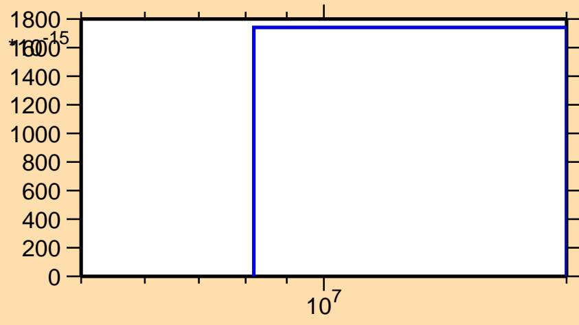
\sigma vs. E for ^{229}\text{Ac}(n,3n\alpha)
