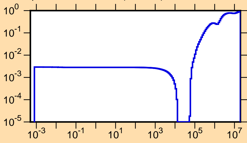
\mu vs. E for ^{230}\text{Ac}(\text{mt251})
