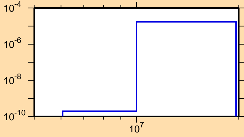
\sigma vs. E for ^{230}\text{Ac}(n,n\alpha)
