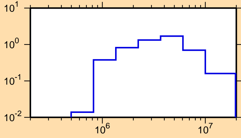
\sigma vs. E for ^{230}\text{Ac}(n,n\text{cont.})
