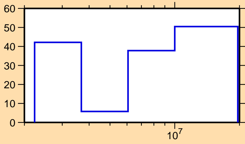
\Delta\sigma/\sigma vs. E for ^{230}\text{Ac}(n,n\text{cont.})
