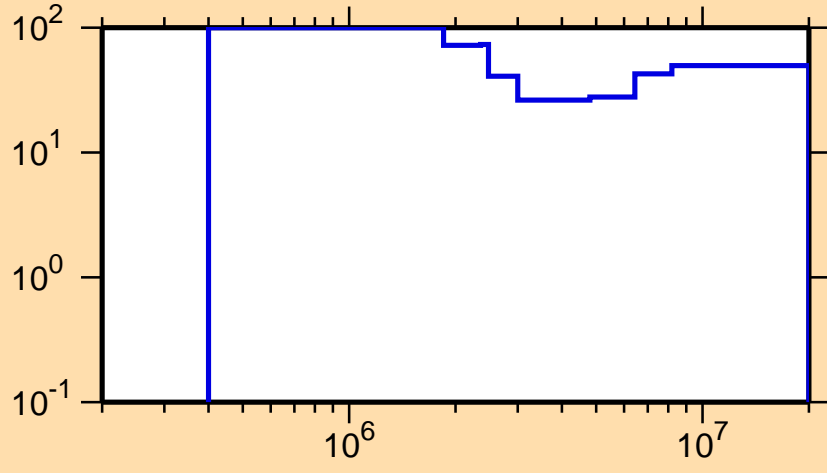
\Delta\sigma/\sigma vs. E for ^{230}\text{Ac}(n,n\text{cont.})
