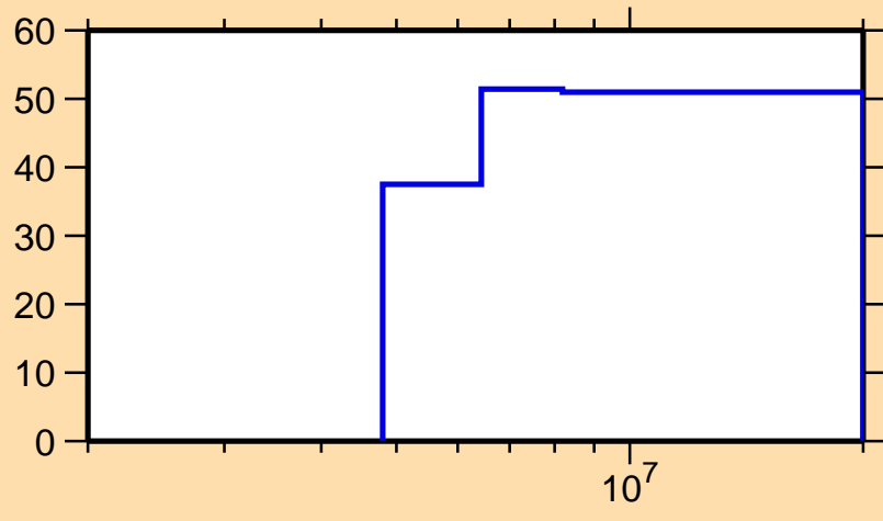
\Delta\sigma/\sigma vs. E for ^{230}\text{Ac}(n,\text{inel.})
