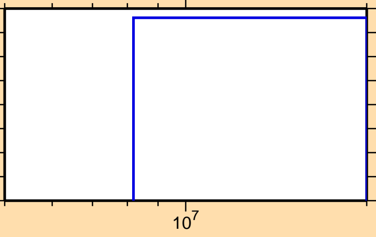
\sigma vs. E for ^{230}\text{Ac}(n,2n\alpha)
