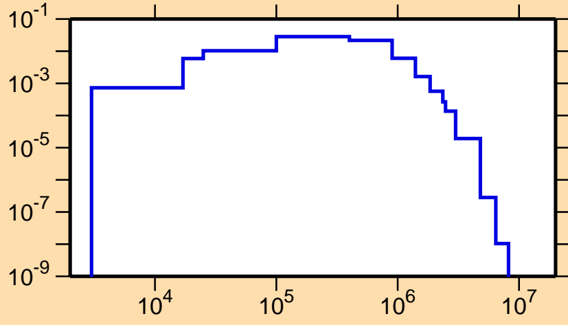
\sigma vs. E for ^{230}\text{Ac}(n,n_1)
