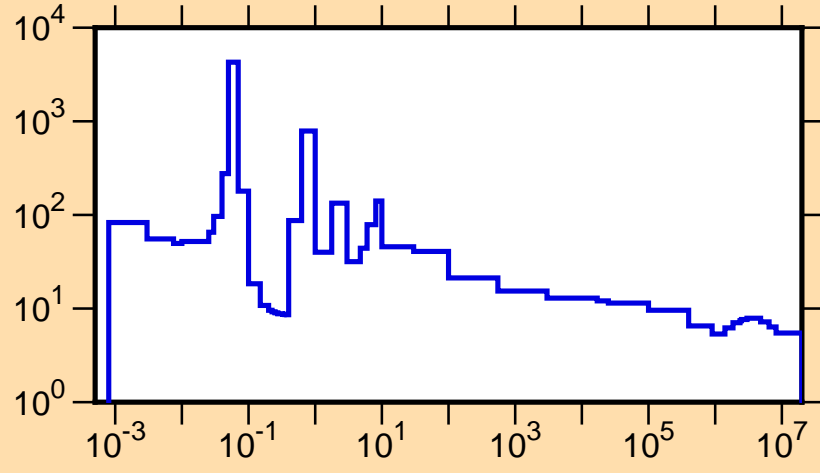
\sigma vs. E for ^{230}\text{Ac}(n,\text{tot.})
