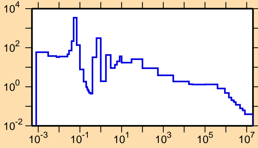
\sigma vs. E for ^{230}\text{Ac}(n,f)
