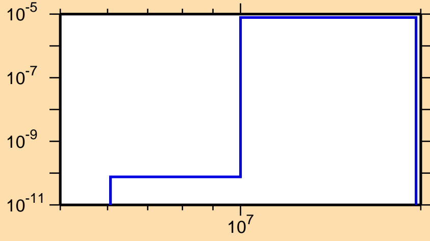
\sigma vs. E for ^{231}\text{Ac}(n,n\alpha)
