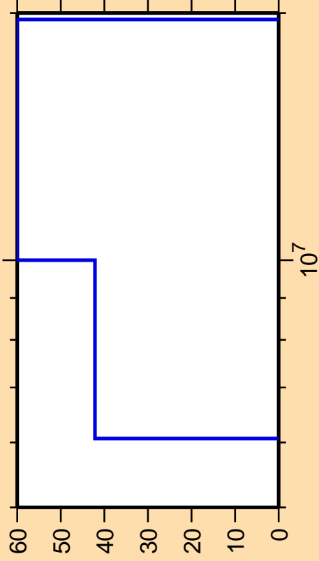
\Delta\sigma/\sigma vs. E for ^{231}\text{Ac}(n,n\alpha)
