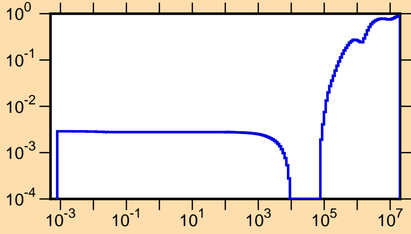
\mu vs. E for ^{232}\text{Ac}(\text{mt251})
