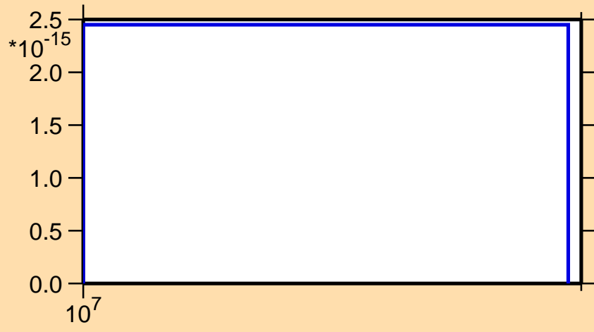
\sigma vs. E for ^{232}\text{Ac} (mt 11)
