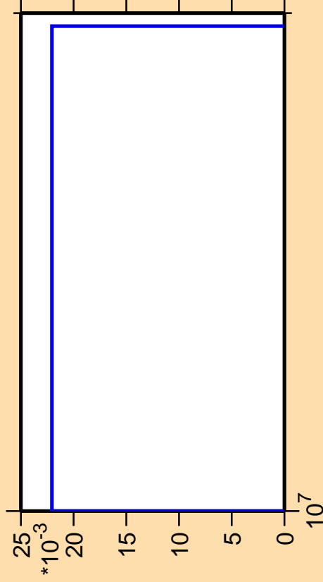
\Delta\sigma/\sigma vs. E for ^{232}\text{Ac} (mt 11)
