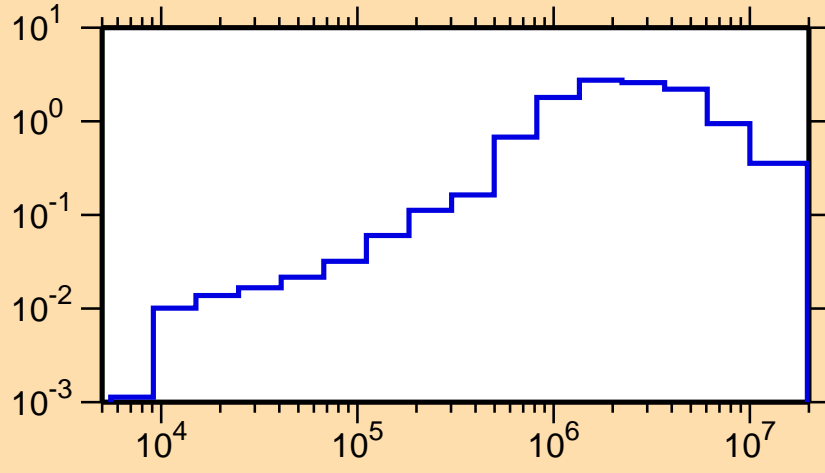
\sigma vs. E for ^{232}\text{Ac}(n,\text{inel.})
