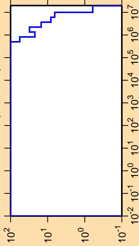
\Delta\sigma/\sigma vs. E for ^{232}\text{Ac}(n,\text{nonel.})
