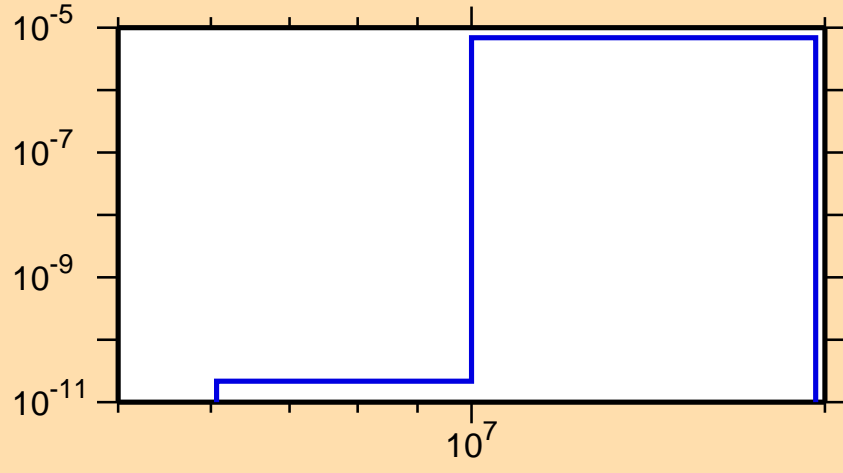
\sigma vs. E for ^{232}\text{Ac}(n,n\alpha)
