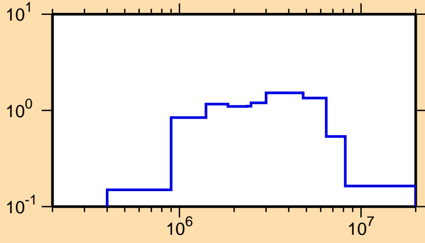
\sigma vs. E for ^{232}\text{Ac}(n,n\text{cont.})
