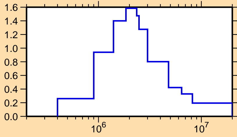
\sigma vs. E for ^{232}\text{Ac}(n,n_3)
