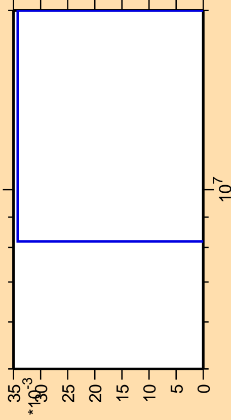
\Delta\sigma/\sigma vs. E for ^{232}\text{Ac}(n,\text{He}3)
