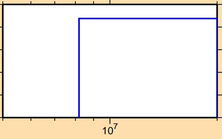
\sigma vs. E for ^{232}\text{Ac}(n,nt)
