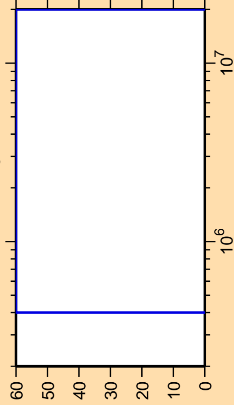
\Delta\sigma/\sigma vs. E for ^{232}\text{Ac}(n,n_3)
