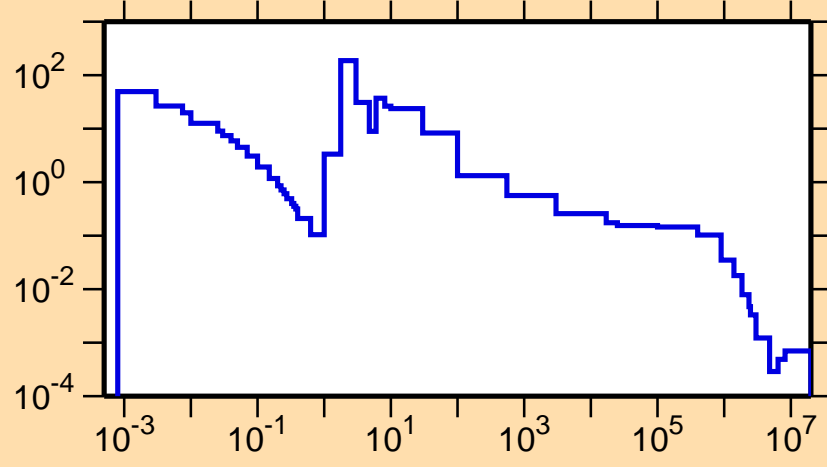
\sigma vs. E for ^{232}\text{Ac}(n,\gamma)
