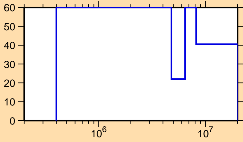
\Delta\sigma/\sigma vs. E for ^{232}\text{Ac}(n,n\text{cont.})
