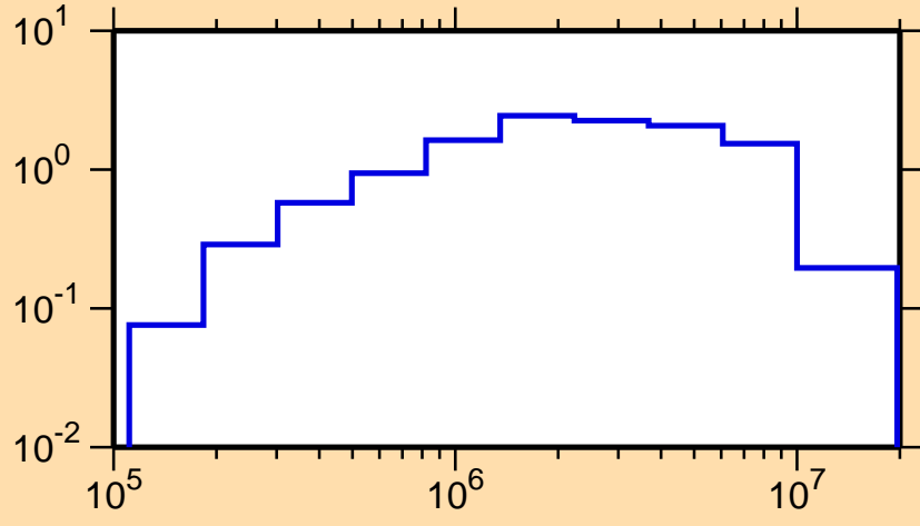
\sigma vs. E for ^{233}\text{Ac}(n,\text{inel.})
