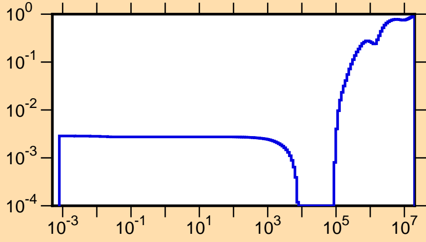
\mu vs. E for ^{234}\text{Ac}(\text{mt251})
