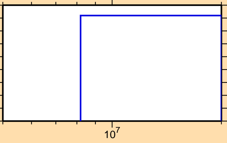
\sigma vs. E for ^{234}\text{Ac}(n,2np)
