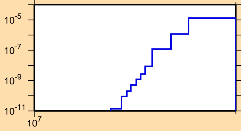
\sigma vs. E for ^{235}\text{Ac}(n,nt)
