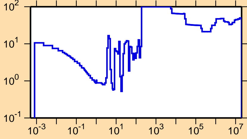
\Delta\sigma/\sigma vs. E for ^{235}\text{Ac}(n,tot.)
