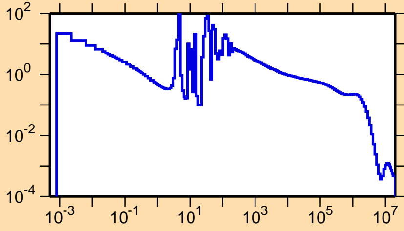
\sigma vs. E for ^{235}\text{Ac}(n,\gamma)
