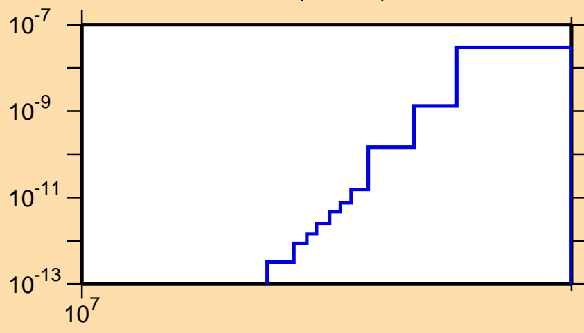
\sigma vs. E for ^{235}\text{Ac}(n,2n\alpha)
