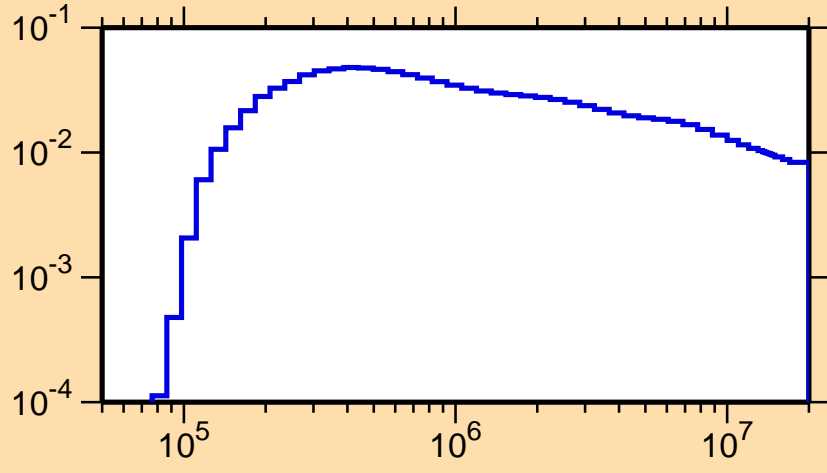
\sigma vs. E for ^{95}\text{Ag}(n,n_1)
