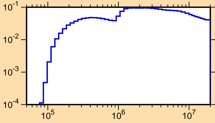
\sigma vs. E for ^{95}\text{Ag}(n,\text{inel.})
