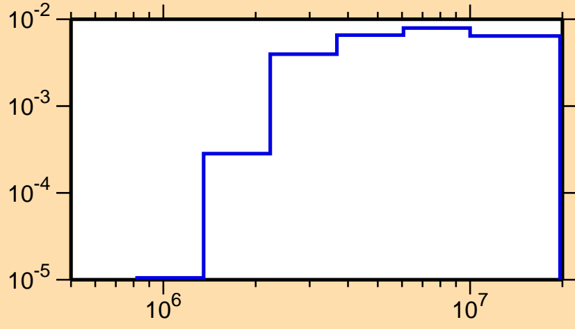
\sigma vs. E for ^{95}\text{Ag}(n,n\text{cont.})
