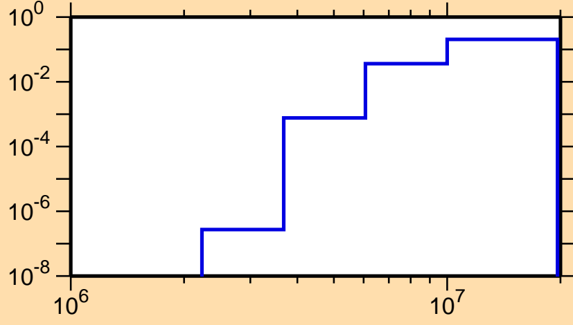
\sigma vs. E for ^{95}\text{Ag}(n,np)
