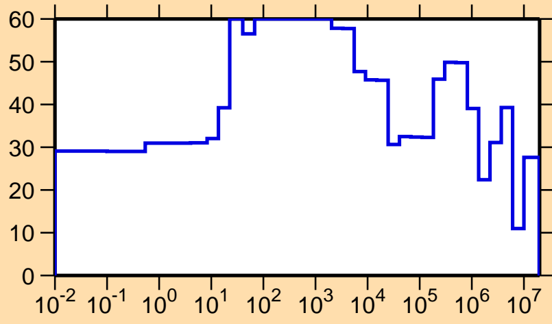
\Delta\sigma/\sigma vs. E for ^{95}\text{Ag}(n,el.)
