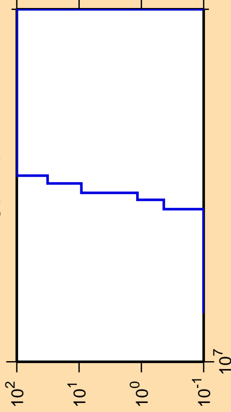
\Delta\sigma/\sigma vs. E for ^{96}\text{Ag}(n,nd)
