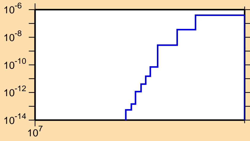
\sigma vs. E for ^{96}\text{Ag}(n,nd)
