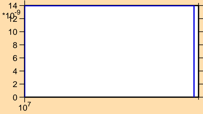
\sigma vs. E for ^{96}\text{Ag} (mt 45)
