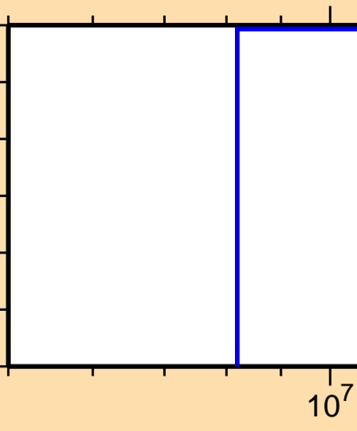
\sigma vs. E for ^{96}\text{Ag}(\text{mt } 45)
