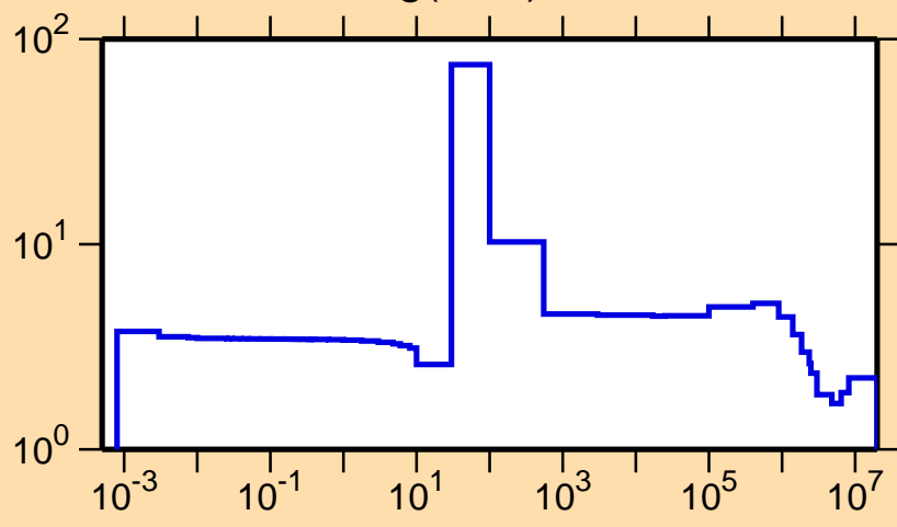
\sigma vs. E for ^{96}\text{Ag}(n,\text{el.})
