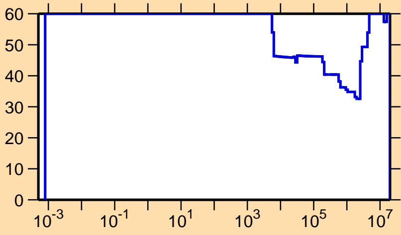
\Delta\sigma/\sigma vs. E for ^{97}\text{Ag}(n,\gamma)
