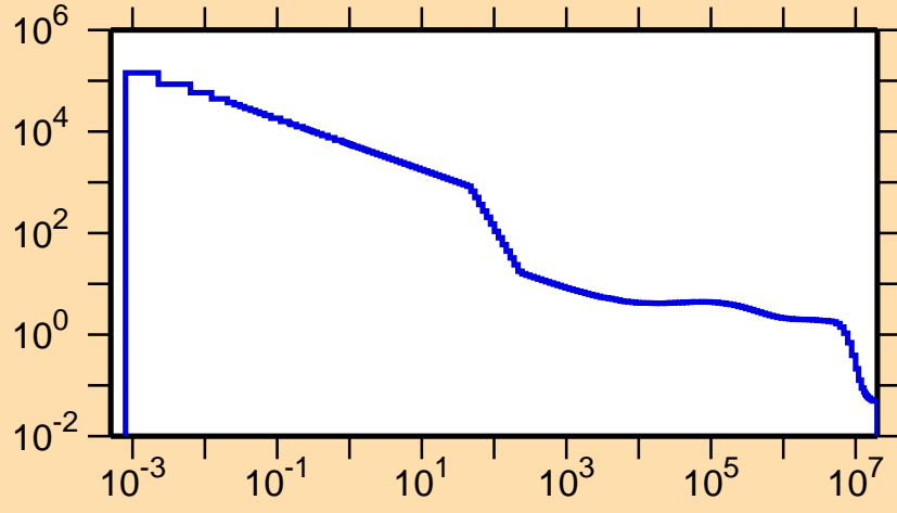
\sigma vs. E for ^{97}\text{Ag}(n,p)
